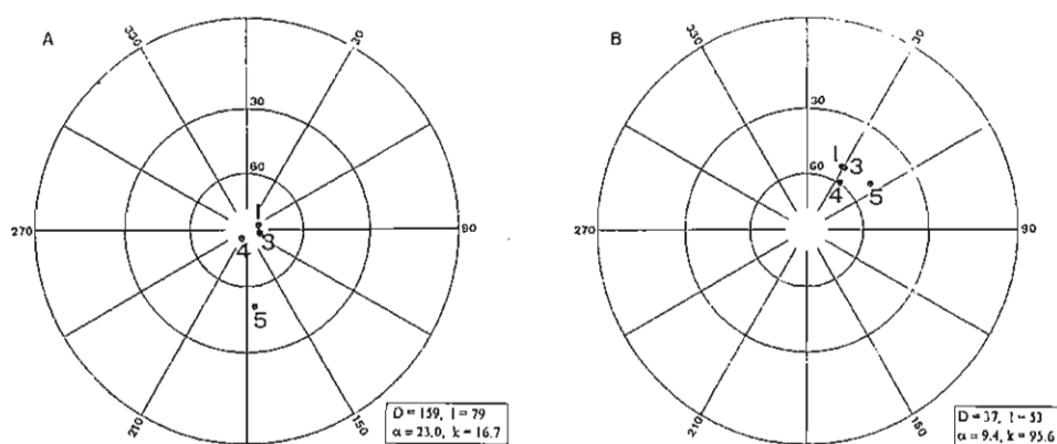
Fig. 5. Fold test for the Bobrowiec unit and the Gładkie Uplaziańskie slice: the characteristic directions from sampled localities (1, 3, 4, 5 — see Fig. 2) before (A) and after (B) tectonic correction
