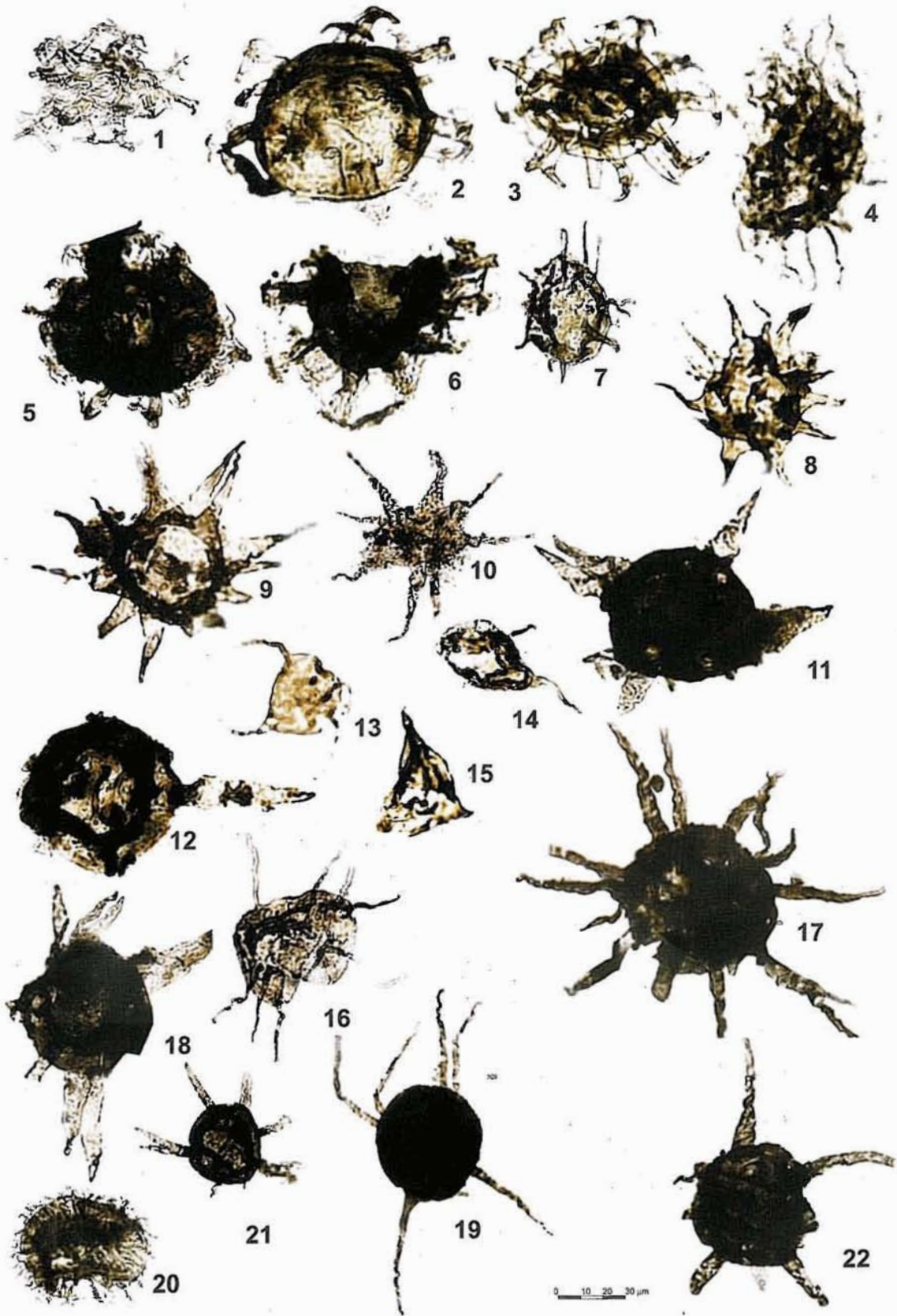
1. Multiplicisphaeridium sp., 2139.7 m. 2, 3. Ordovicidium elegantulum Tappan et Loeblich, 2139.7 m. 4. Baltisphaeridium annelienae (Kjellström), 2139.7 m. 5. Peteinosphaeridium trifurcatum (Eisenack), 2597.3 m. 6. Peteinosphaeridium sp., 2141.0 m. 7. " Goniosphaeridium " cf. smedsbiense Görka, 2141.0 m. 8, 9. Polygonium gracile Vavrdová: 8—2139.7 m, 9—2520.7 m. 10. Polygonium sp., 2111.0 m. 11. Baltisphaeridium cf. bramkaense Görka, 2597.3 m. 12. Baltisphaeridium bramkaense Görka, 2597.3 m. 13. Veryhachium sp., 2111.0 m. 14. Veryhachium cf. hamii Loeblich, 2113.0 m. 15. Veryhachium reductum (Dcunff), 2113.0 m. 16, 19. Baltisphaeridium longispinosum (Eisenack), 2111.0 m. 17, 22. Baltisphaeridium plicatispinae Görka, 2520.7 m. 18. Baltisphaeridium lancettispinae Görka, 2520.7 m. 20. ? Multiplicisphaeridium sp., 2111.0 m. 21. Baltisphaeridium calicispinae Görka, 2428.0 m. Jamno IG 2 borchole
