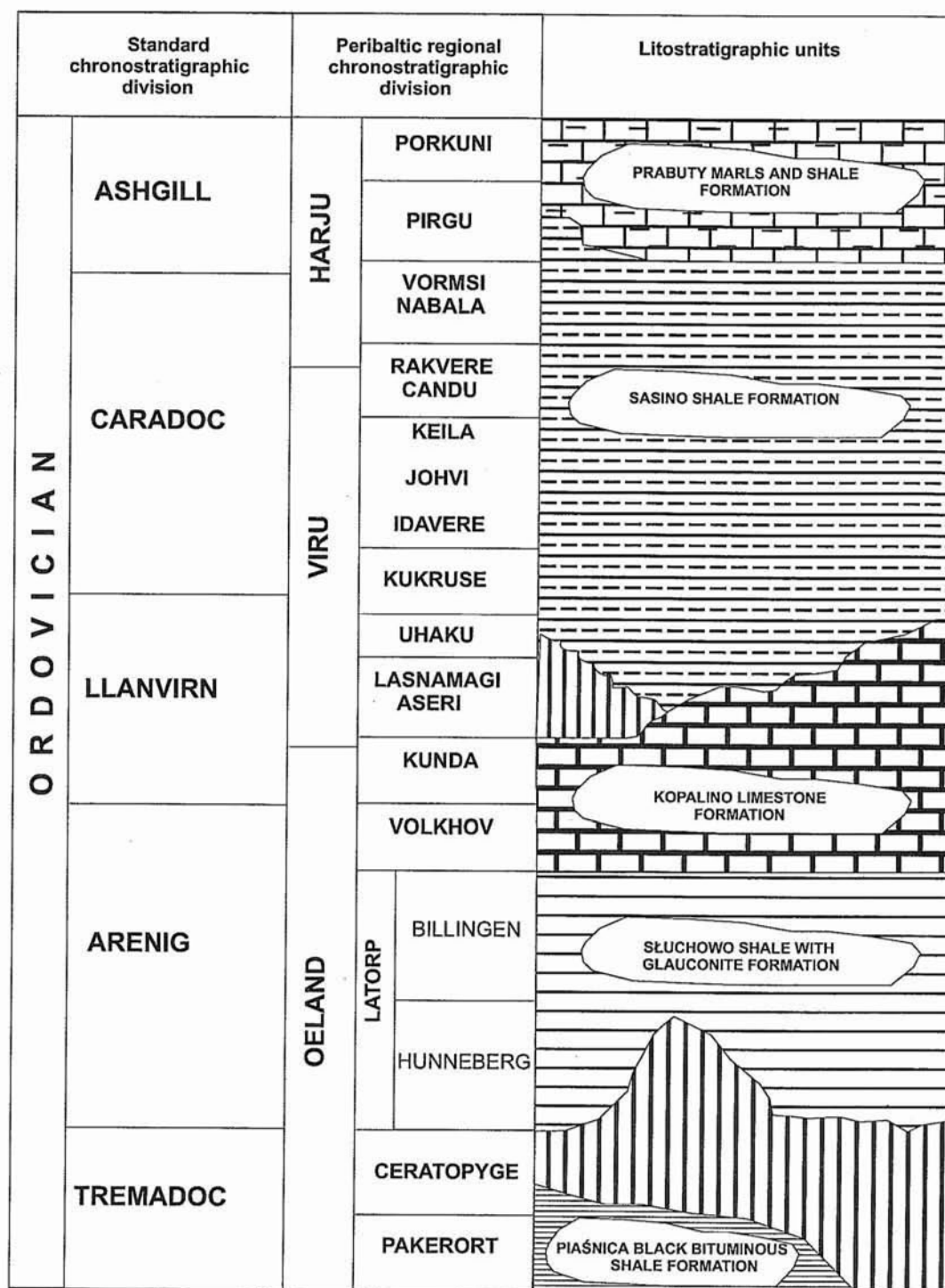
Fig. 2. Ordovician lithostratigraphical scheme in the western part of the Peribaltic Syncline, after Modliński and Szymański (1997), simplified
