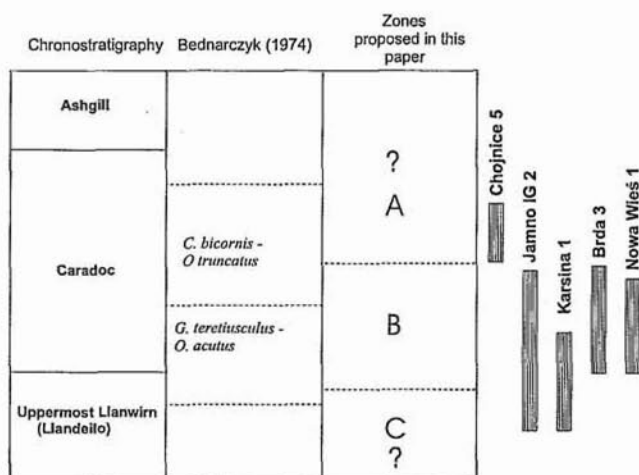
Fig. 4. Correlation scheme of local palaeontological zones in the Ordovician of the Pomeranian Caledonides
