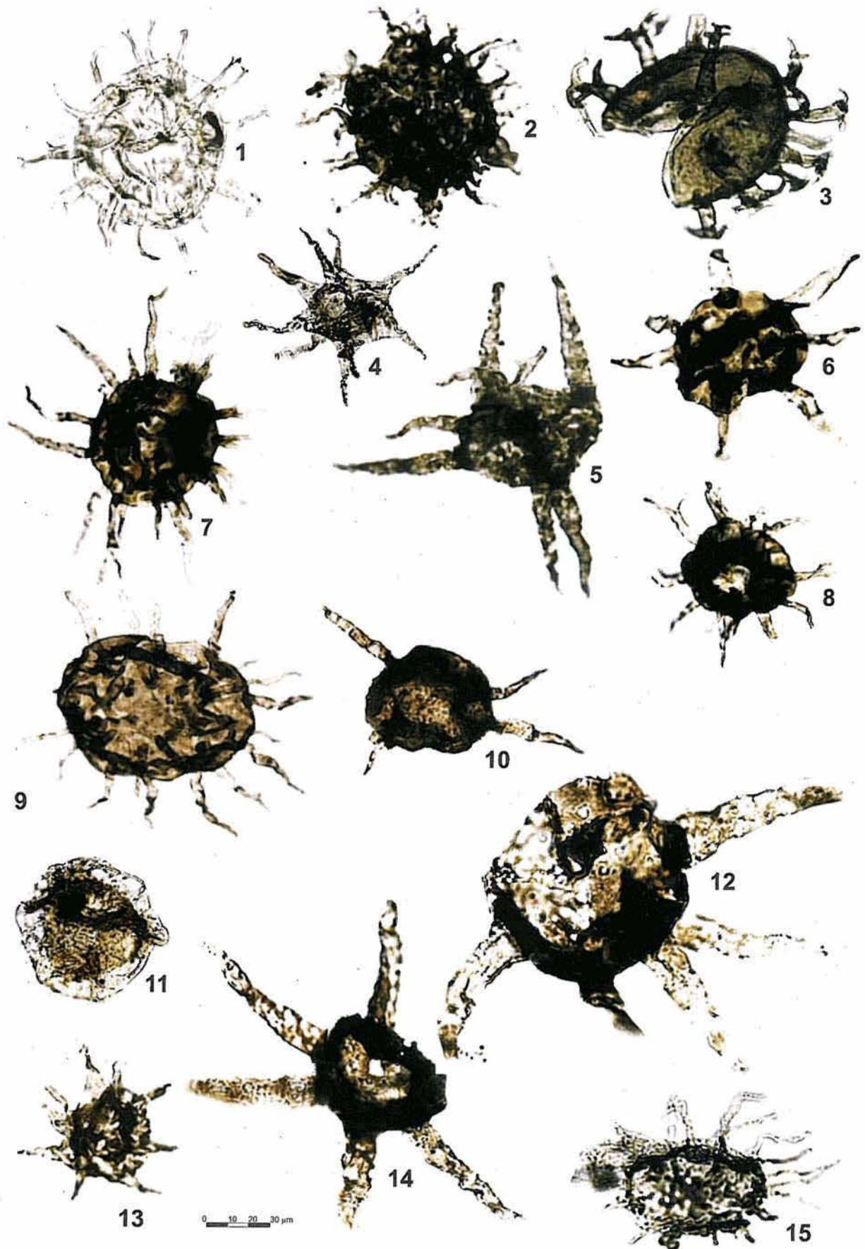
1. Exculibranchium sp., 3201.5 m. 2. Multiplicisphaeridium sp., 3140.0 m. 3. Ordovicidium nudum (Eisenack), 3166.0 m. 4, 13. Polygonium gracile Vavrdová: 4 — 3166.0 m, 13 — 3201.5 m. 5. Gorgoniosphaeridium sp., 3140.0 m. 6. Baltisphaeridium lancettispinae Görka, 3166.0 m. 7, 9. Baltisphaeridium plicatispinae Görka: 7 — 3140.5 m, 9 — 3140.0 m. 8. Baltisphaeridium cf. hirsutoides (Eisenack), 3166.0 m. 10. Baltisphaeridium sp., 3166.0 m. 11. ? Cymatiogalea sp., 3140.0 m. 12. Baltisphaeridium cf. lancettispinae Görka, 3201.5 m. 14. Baltisphaeridium calicispinae Görka, 3166.0 m. 15. ? Baltisphaeridium sp., 3166.0 m. Karsina 1 borehole
