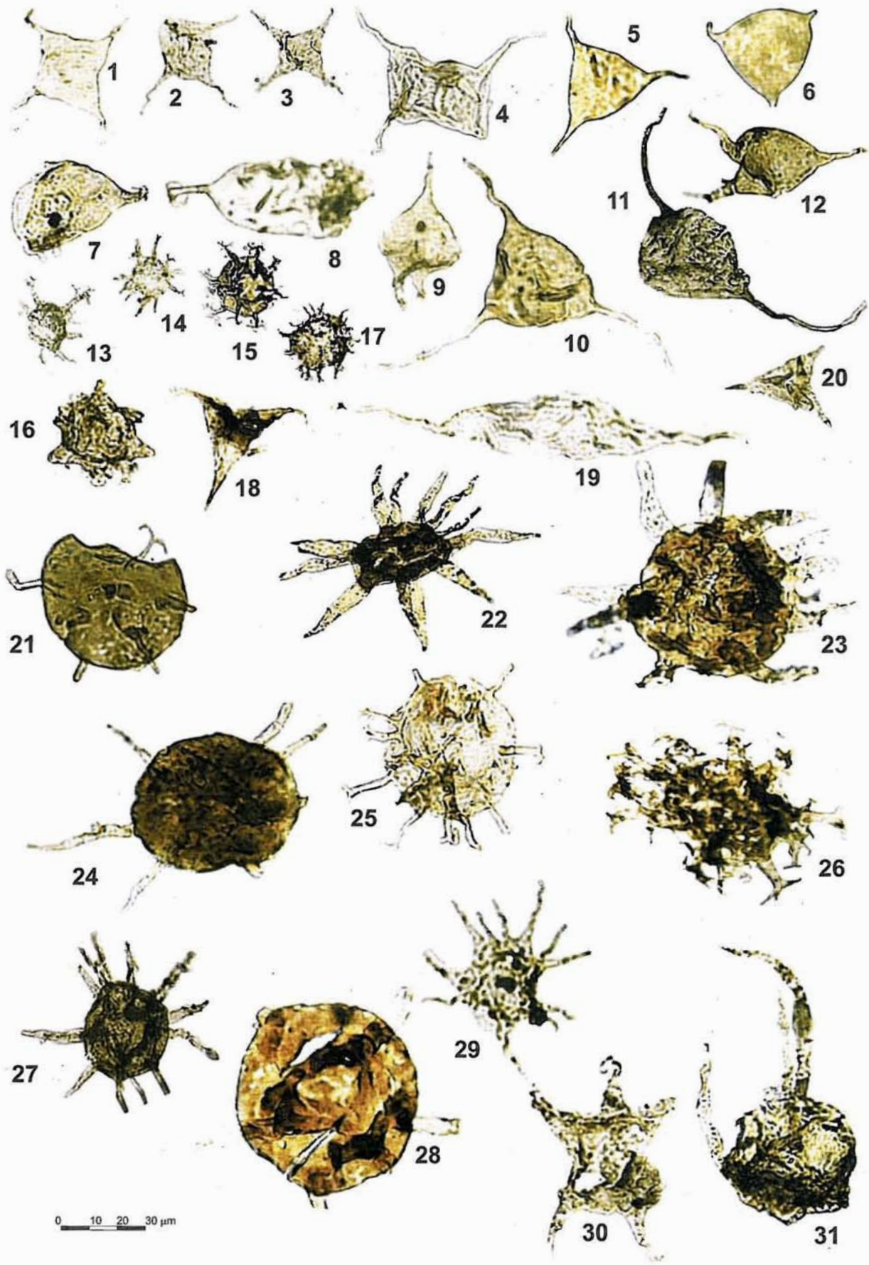
1, 3, 4. Veryhachium oklahomense (Loeblich): 1, 4 — 2153.4 m, 3 — 2900.5 m. 2. Veryhachium cf. oklahomense (Loeblich), 2900.5 m. 5, 10. Veryhachium trispinosum (Eisenack), 2153.4 m. 6. Veryhachium reductum (Deunff), 2153.4 m. 7, 8. Pirea sp., 2153.4 m. 9, 12. ? Veryhachium sp.: 9 — 2153.4 m, 12 — 2900.5 m. 11, 19. Leiofusa sp.: 11 — 2900.5 m, 19 — 2153.4 m. 13, 14, 17. ? Multiplicisphaeridium sp.: 13 — 2900.5 m, 14 — 2153.4 m, 17 — 2643.5 m. 15, 25. Exculibranchium sp., 2153.4 m. 16. Petaloferidium sp., 2153.4 m. 18, 20. Veryhachium trispinosum ssp. geometricum Deflandre, 2643.5 m. 21. Ordovicidium heteromorphum (Kjellström), 2153.4 m. 22. Baltisphaeridium latiradiatum (Eisenack), 2643.5 m. 23. Baltisphaeridium brevispinosum (Eisenack), 2153.4 m. 24. Baltisphaeridium calicispinae Gôrka, 2153.4 m. 26. Multiplicisphaeridium sp., 2643.5 m. 27. Baltisphaeridium cf. hirsutoides (Eisenack), 2900.5 m. 28. Actipilon cf. druggi Loeblich, 2153.4 m. 29. Polygonium gracile Vavrdová, 2153.4 m. 30. Polygonium sp., 2643.5 m. 31. ? Gorgoniosphaeridium sp., 2643.5 m. Brda 3 borhole
