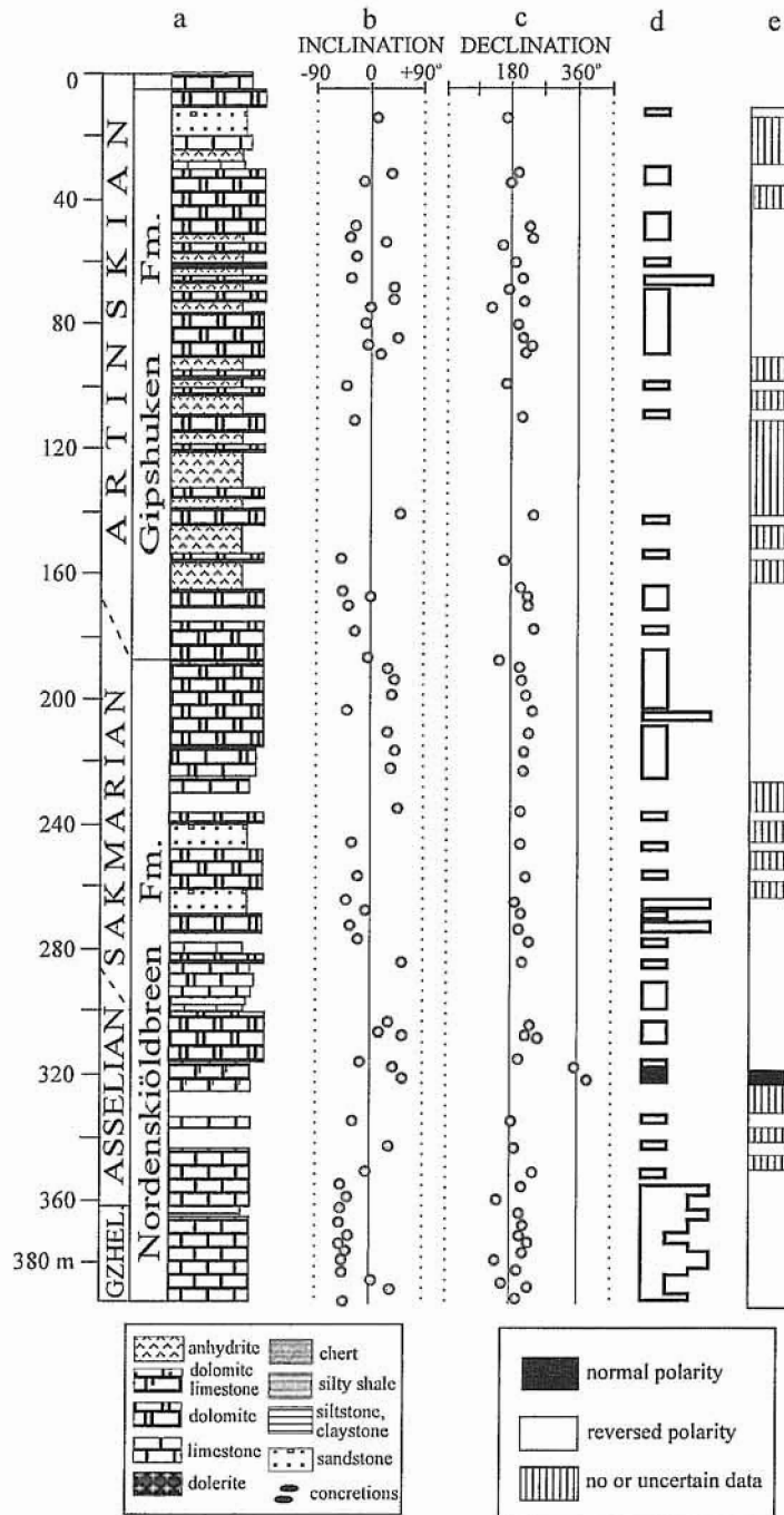
Fig. 4. Lithological column and stratigraphy (a), inclination (b) and declination (c) graphs, polarity pattern graphs (d) and composite polarity scale (e) constructed for the Late Gzhelian-Artinskian formations from Kapp Schoultz locality
