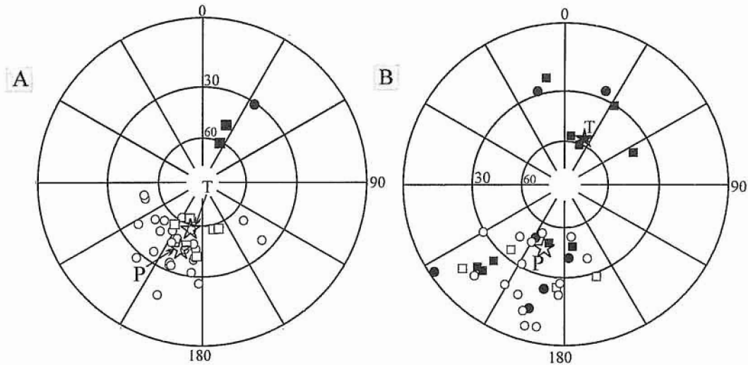
Fig. 3. A — stereographic projection of the Late Gzhelian-Permian (circles) and Griesbachian (squares) line-fit directions from Kapp Schoultz and Trygghamna sections; B — stereographic projection of the directions obtained on the terminus levels of thermal demagnetisation (before rapid increase of magnetic susceptibility at temperatures of about 425°C) of the Late Gzhelian-Artinskian (locality Kapp Schoultz) and Early Triassic (locality Tschermakfjellet) partly remagnetised samples; the asterisks with the letters P and T show the mean Permian and Triassic direction respectively; in stereoplots, open (closed) symbols denote upward (downward) pointing inclinations
