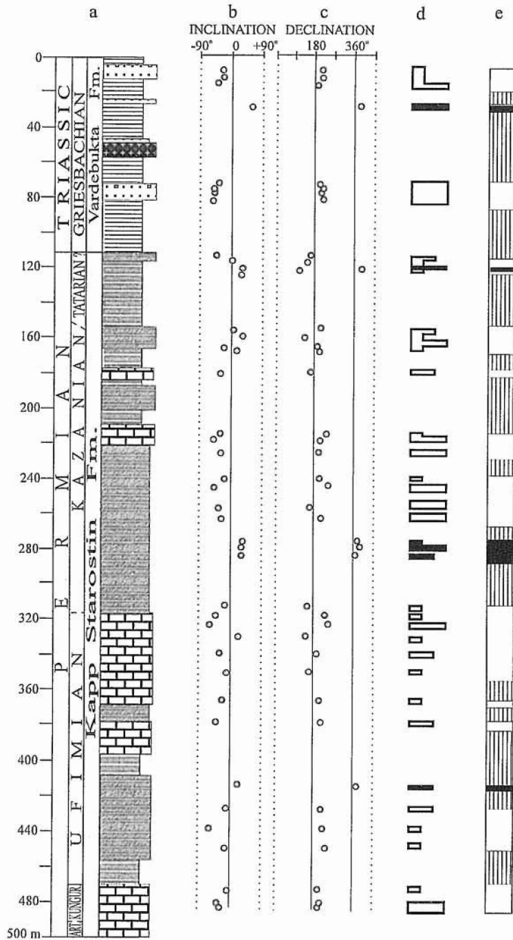
Fig. 5. Lithological column and stratigraphy (a), inclination (b) and declination (c) graphs, polarity pattern graphs (d) and composite polarity scale (e) constructed for the Late Artinskian-Griesbachian formations from Trygghamna locality
