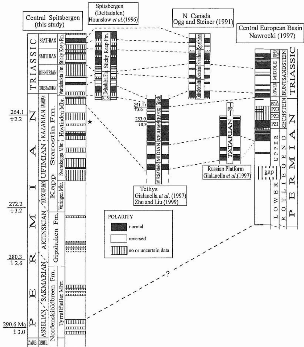
Fig. 7. Composite Late Gzhelian-Spathian polarity scale for central Spitsbergen and its correlation with magnetostratigraphy from other localities
