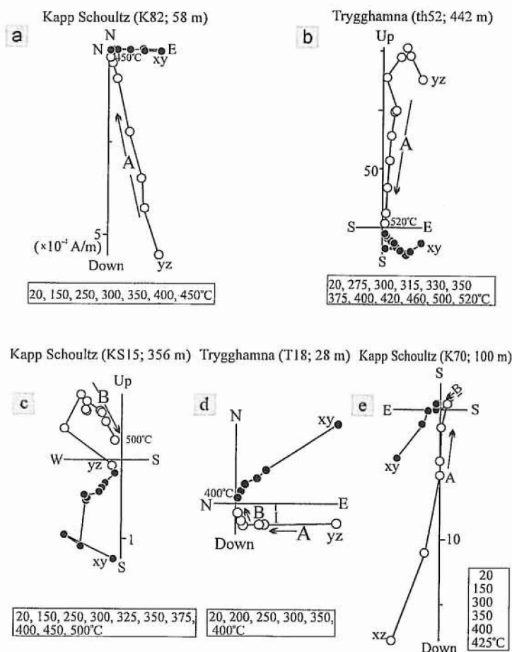
Fig. 2. Orthogonal demagnetograms of representative samples of Late Gzhelian-Early Triassic rocks from central Spitsbergen
