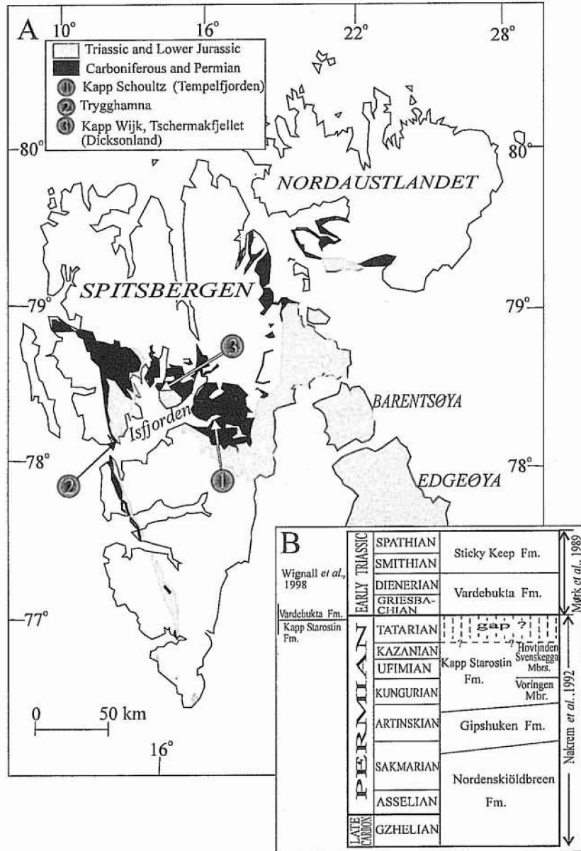
Fig. 1. A — Carboniferous-Lower Jurassic outcrop areas in the Svalbard Archipelago (after Mørk et al. , 1989; Nakrem et al. , 1992); regions of palaeomagnetic investigations have been marked by arrows; B — Late Carboniferous-Early Triassic stratigraphy in Spitsbergen; continuous (Wignall et al. , 1998) or discontinuous (Nakrem et al. , 1992) nature of Permian-Triassic boundary are illustrated
