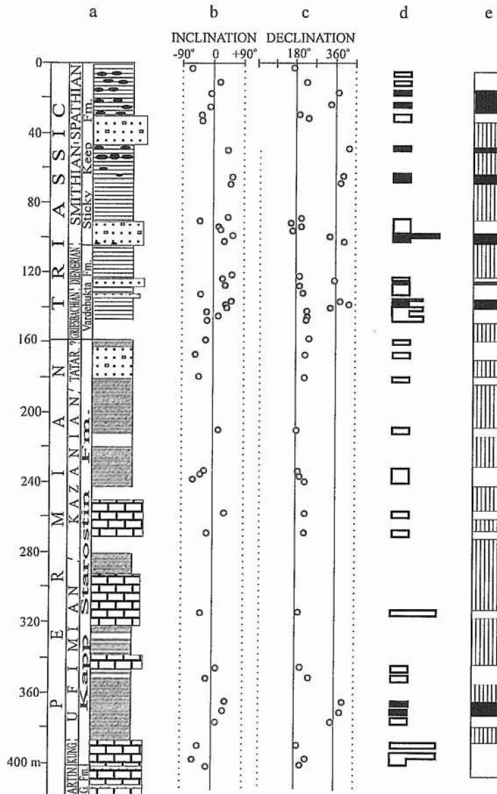
Fig. 6. Lithological column and stratigraphy (a), inclination (b) and declination (c) graphs, polarity pattern graphs (d) and composite polarity scale (e) constructed for the Late Artinskian-Spathian formations from Kapp Wijk, Tschermakfjellet localities
