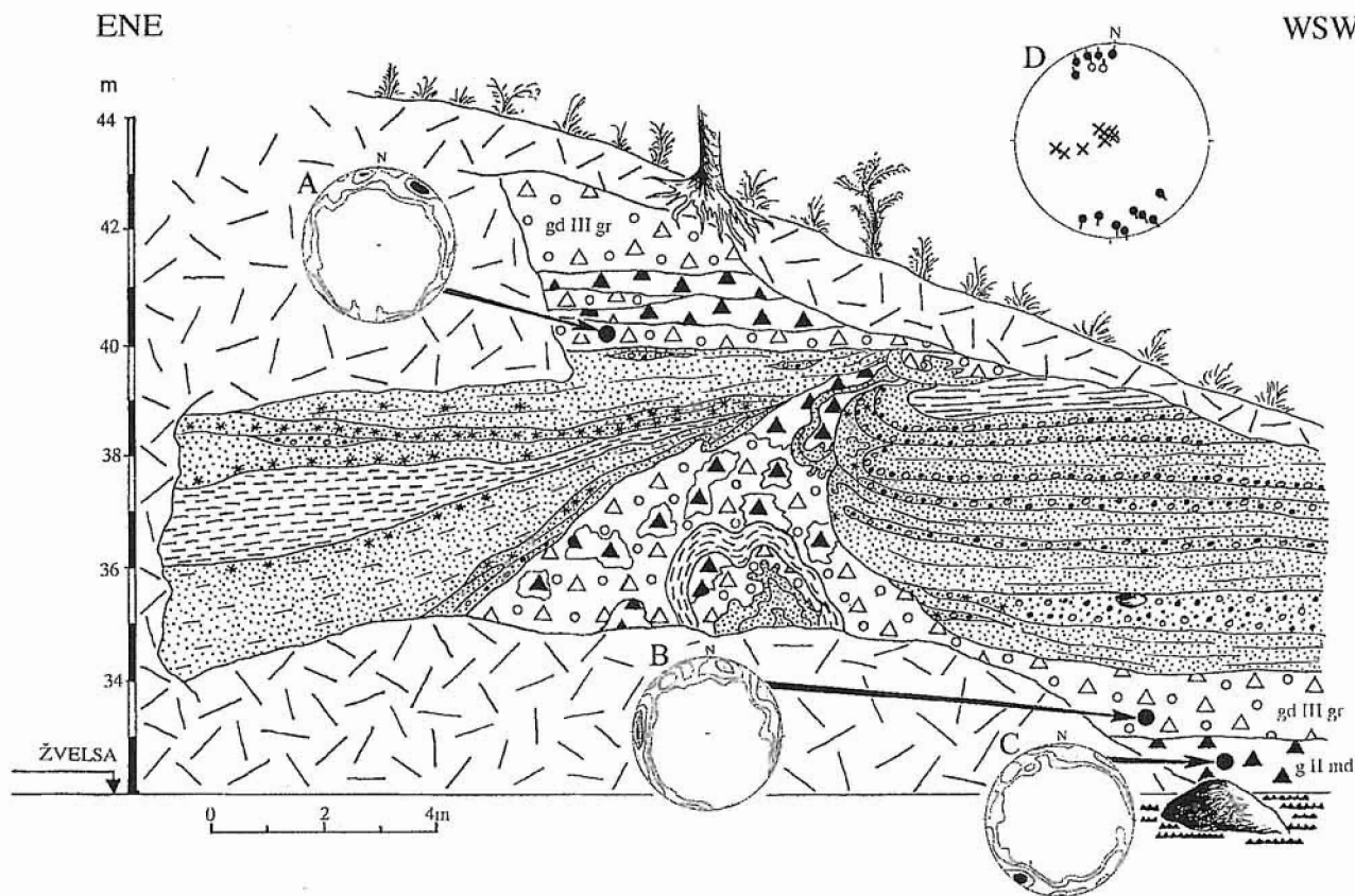
Fig. 3. Glacioidislocations in the outcrop on the left side of the Žvelsa Creek close to Lapiai in the Klaipėda District, western Lithuania
