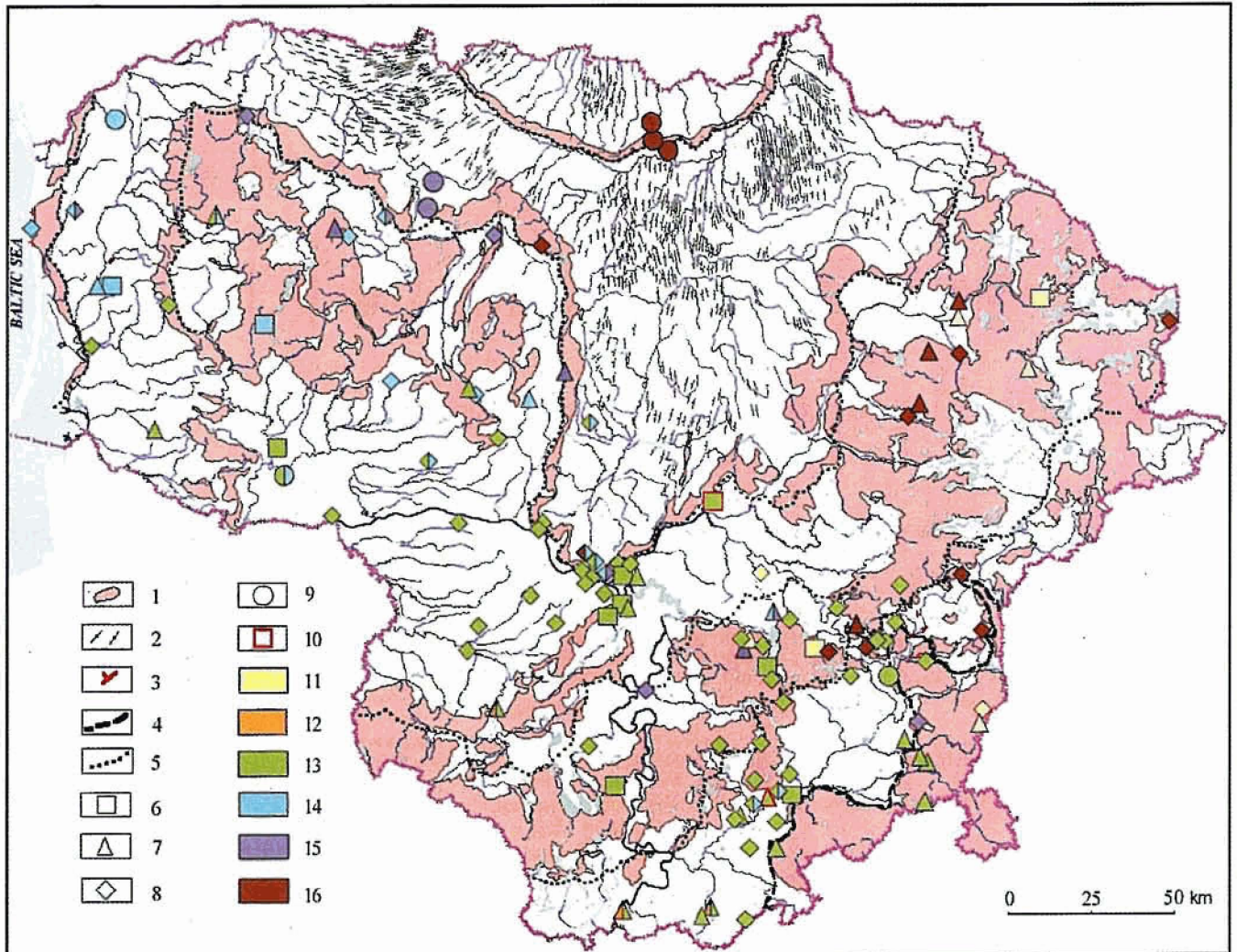
Fig. 1. Glaciotectonic review map of Lithuania, compiled on the basis of the Quaternary Geological Map of Lithuania (Guobytė, 1998) and the Geomorphological Map of the Soviet Baltic Republics (Straume, 1980)
