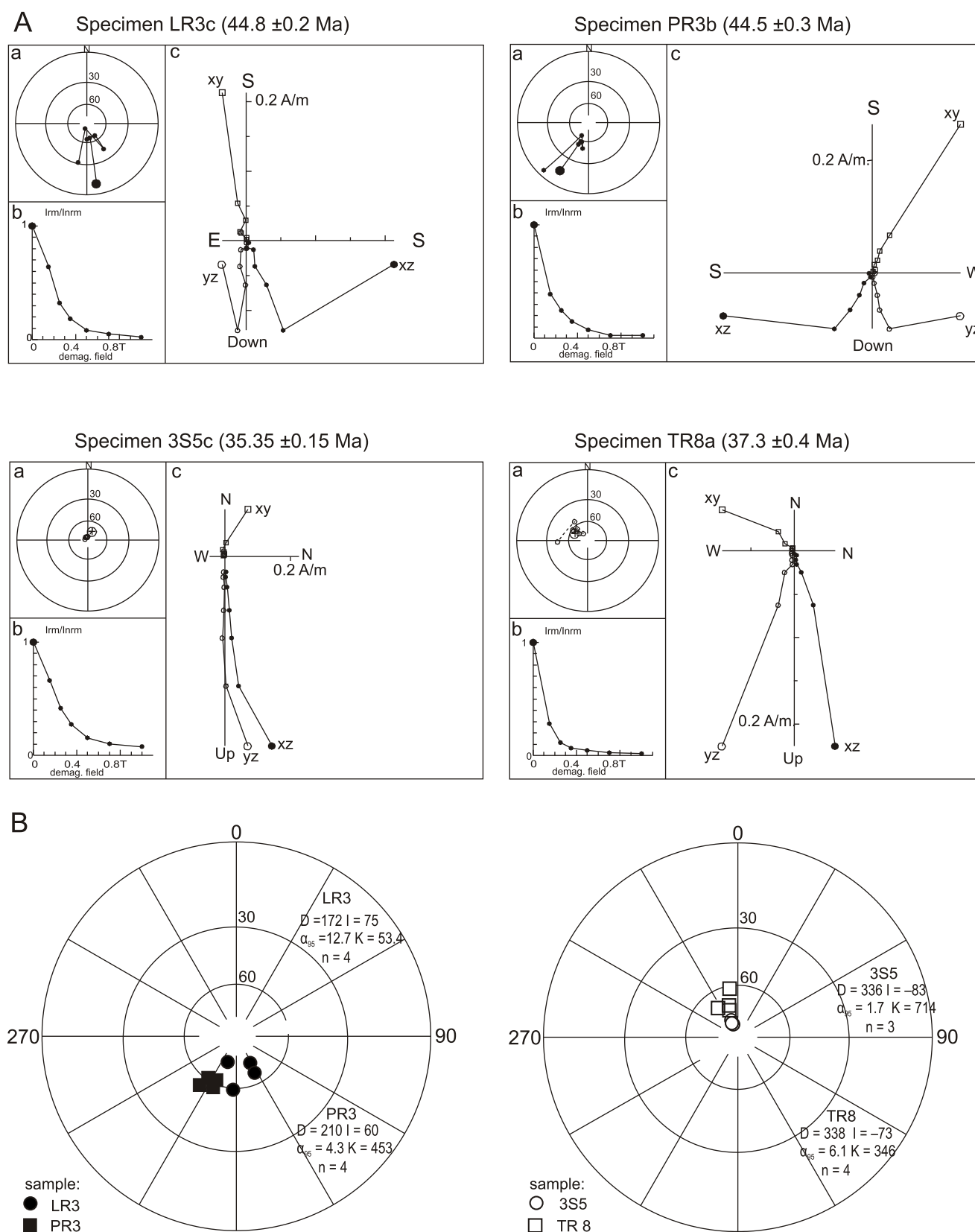
Fig. 8A – typical demagnetisation characteristics (a – demagnetisation paths, b – intensity decay curves, c – orthogonal plots) of the volcanic rocks from the Lions Rump area (Batke Point – LR3c; Polish Geological Survey Cliff – PR3b), Turret Point (TR8a) and Three Sisters Point (3S5c) section; B – stereographic projections of line-fit mean (on the specimen level) palaeomagnetic directions isolated from the Lions Rump area (Batke Point – LR3c; Polish Geological Survey Cliff – PR3b), Turret Point (TR8a) and Three Sisters Point (3S5c); the diagrams were prepared by means of a computer package developed by Lewandowski et al. (1997)
