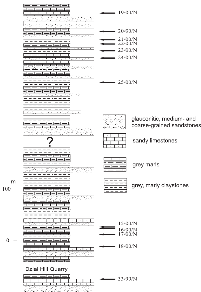
Fig. 7. Lithostratigraphical log of the Zawada Formation in the Poręba Mała area
