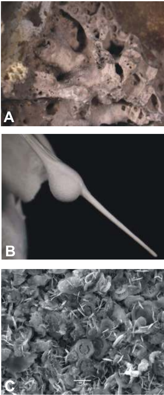
Fig. 11A — vesicular mass of stalactitic-like godovikovite, field of view 1.4 cm; B — nodosity in a godovikovite stalactite, field of view 2.4 cm; C — pseudohexagonal blades of godovikovite, SEM image
