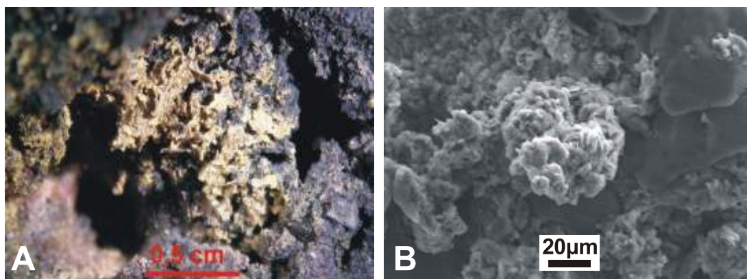
Fig. 9A — clairite-bearing assemblage from Czerwionka-Dębieńsko; B — clairite rosette by rounded boussingaultite, SEM image
