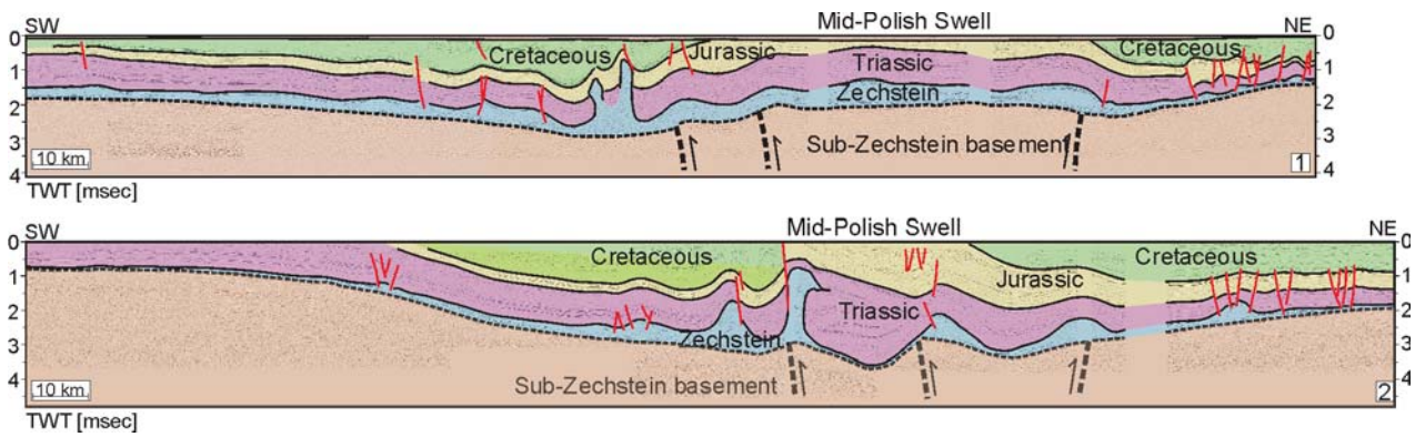
Fig. 3. Regional seismic profiles across the Pomeranian (1) and the Kuiavian (2) segments of the inverted Mid-Polish Trough (after Krzywiec, 2004a, 2006; Krzywiec et al. , 2006)
