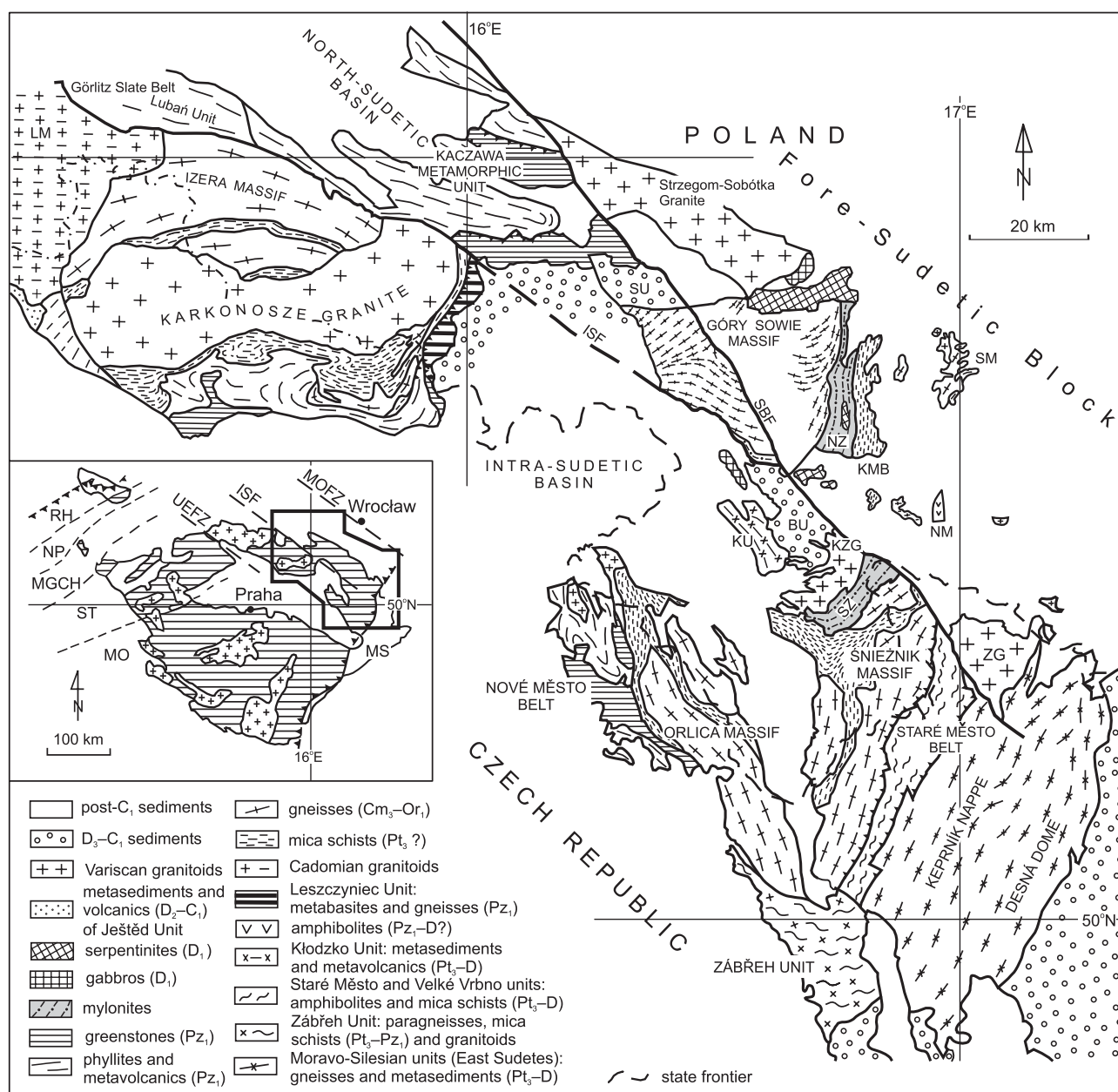
Fig. 3. Geological sketch map of the Sudetes (after Aleksandrowski et al. , 1997)
