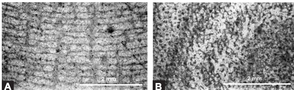
Fig. 4. Actinostroma cf. crassepilatum Lecompte, 1951 from the Early Frasnian Wietrznia Beds at Śluchowice quarry (see Fig. 1D); A — longitudinal section, B — obliquely-tangential section
