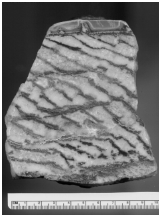
Fig. 7. Banded calcite vein displaying apparent internal tectonic S–C fabrics (Kohút, 1989)
