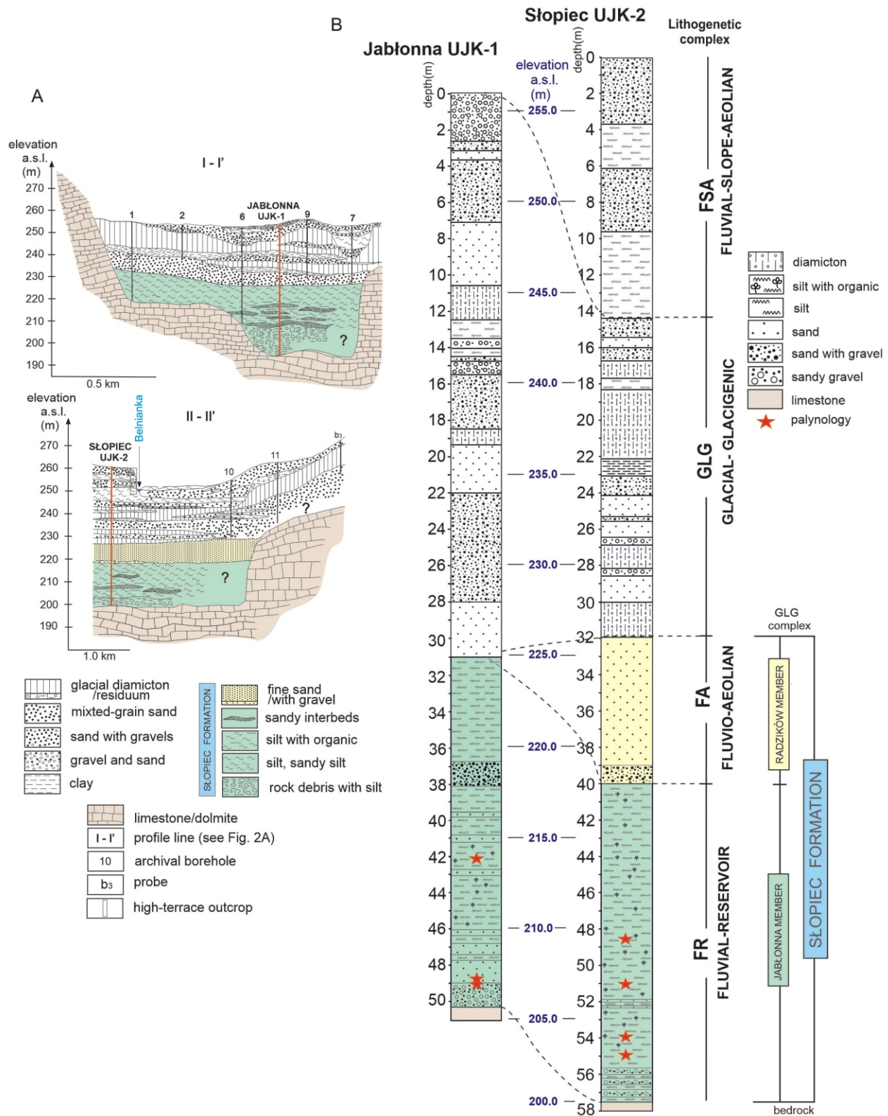
Fig. 2A – geological cross-sections through Quaternary deposits in the Jabłonna and Słópiec area (according Ludwikowska-Kędzia, 2018 , modified); B – lithological profiles of the Jabłonna UJK-1 and Słópiec UJK-2 boreholes (according Ludwikowska-Kędzia, 2018 )
