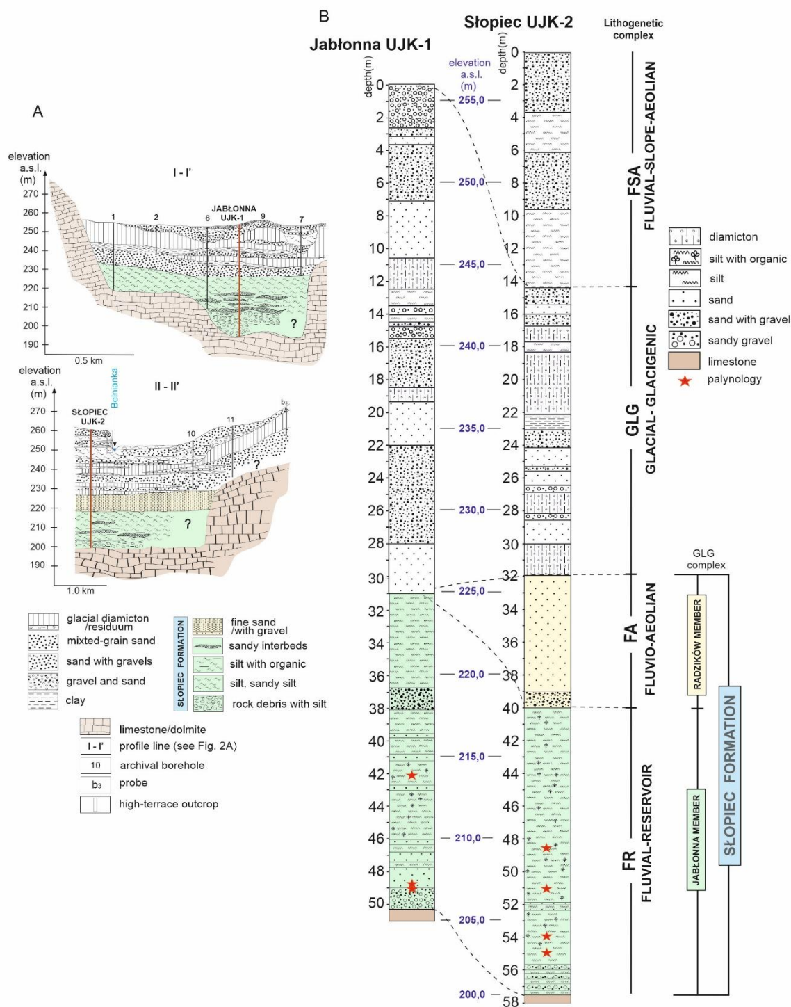
Fig. 2. A. Geological cross-sections through Quaternary deposits in the Jabłonna and Słopiec area (according Ludwikowska-Kędzia, 2018, modified), B. Lithological profiles of the Jabłonna UJK-1 and Słopiec UJK-2 boreholes (according Ludwikowska-Kędzia, 2018)
