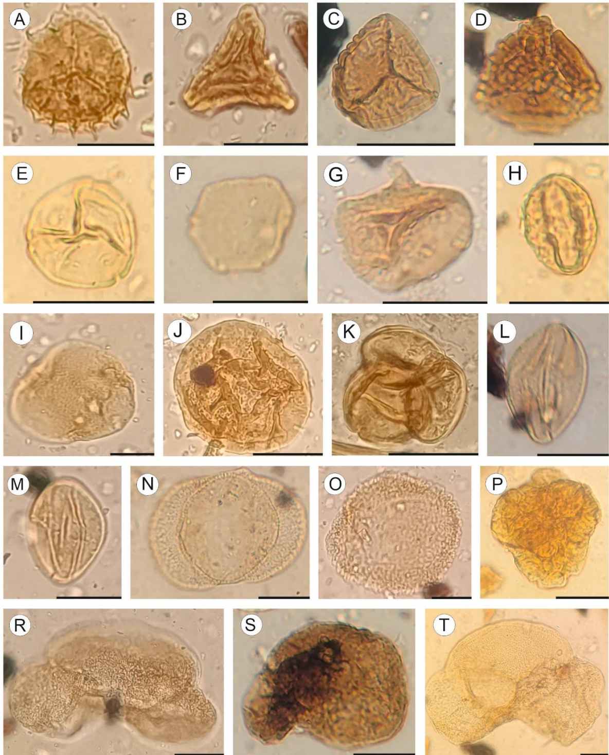
Fig. 8. Palynomorph specimens from the Jabłonna Member (Słupiec UJK–2 borehole), depth 48.5 m. A – Retitriteles sp., B – Neogenisporis neogenicus Krutzsch, C – Camarozonosporites heskemensis (Pflanzl) Krutzsch, D – Cicatricosisporites paradorogensis Krutzsch, E – Myricipites bituitus (Potonié) Nagy, F – Pterocaryapollenites sp., G. Sequoiapollenites sp., H – Cupuliferoipollenites pusillus (Potonié) Potonié, I – Intratiporopollenites inculptus Mai, J – Leiosphaeridia sp., K – Ericipites , L – Tricolporopollenites pseudocingulum (Potonié) Thomson & Pflug, M – Quercoidited henrici (Potonié) Potonié, Thomson & Thiergart, N – Cathayapollis sp., O – Zonalapollenites sp., P. Botryococcus sp., R – Abiespollenites sp., damaged, S – Pre-Cenozoic Pinaceae, T – Abiespollenites sp.
