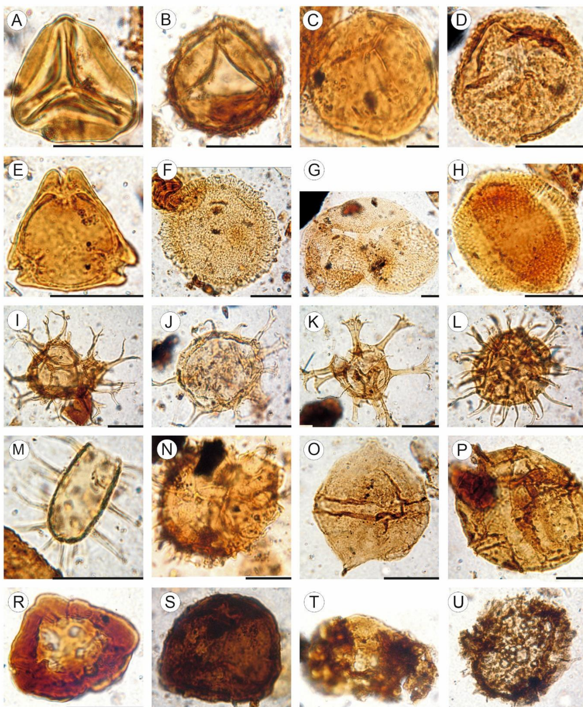
Fig. 7. Palynomorph specimens from the Jabłonna Member (Słopiec UJK-2 borehole), depth 51.0 m. A – Neogenisporis crassicus Krutzsch, B – Rudolphisporis major (Stuchlik) Stuchlik, C – cf. Rugulatisporites , D – Baculatisporites primaries (Wolf) Pflug & Thomson, E – Trudopollis sp., F – Zonalapollenites sp., G – Pinuspollenites sp., H – Crassosphaera sp., I – Spiniferites sp., J – Achomosphaera alcornu (Eisenack) Davey & Williams, K – Cordosphaeridium cf. inodes , L – Operculodinium cf. tiara , M – Tanyosphaeridium sp., N – cf. Glaphyrocysta , O – cf. Spinidinium , P – cf. Cribroperidinium , R., S – Pre-Cenozoic cryptogams, T – Pre-Cenozoic Pinaceae, U – unidentified phytoplankton
