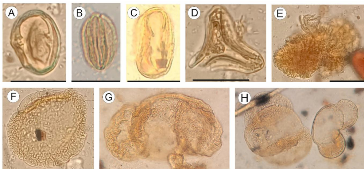
Fig. 9. Palynomorph specimens from the Jabłonna Member (Jabłonna UJK.1 borehole), depth 42.2 m. A – Nyssapollenites sp., B – Quercopollenites sp., C – Tricolporopollenites dolium (Potonié) Thomson & Pflug, D – Neogenisporis neogenicus , E – Botryococcus sp., F – Zonalapollenites sp., G – Pinaceae, damaged, H – left specimen – Abiespollenites sp.; right specimen – Pinuspollenites
