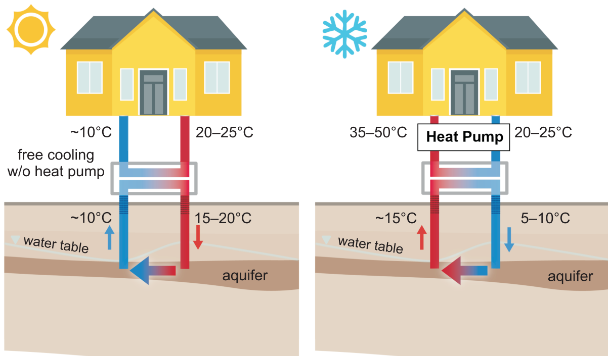
Fig. 1. Simplified scheme of LT-ATES systems operation in summer and winter seasons
