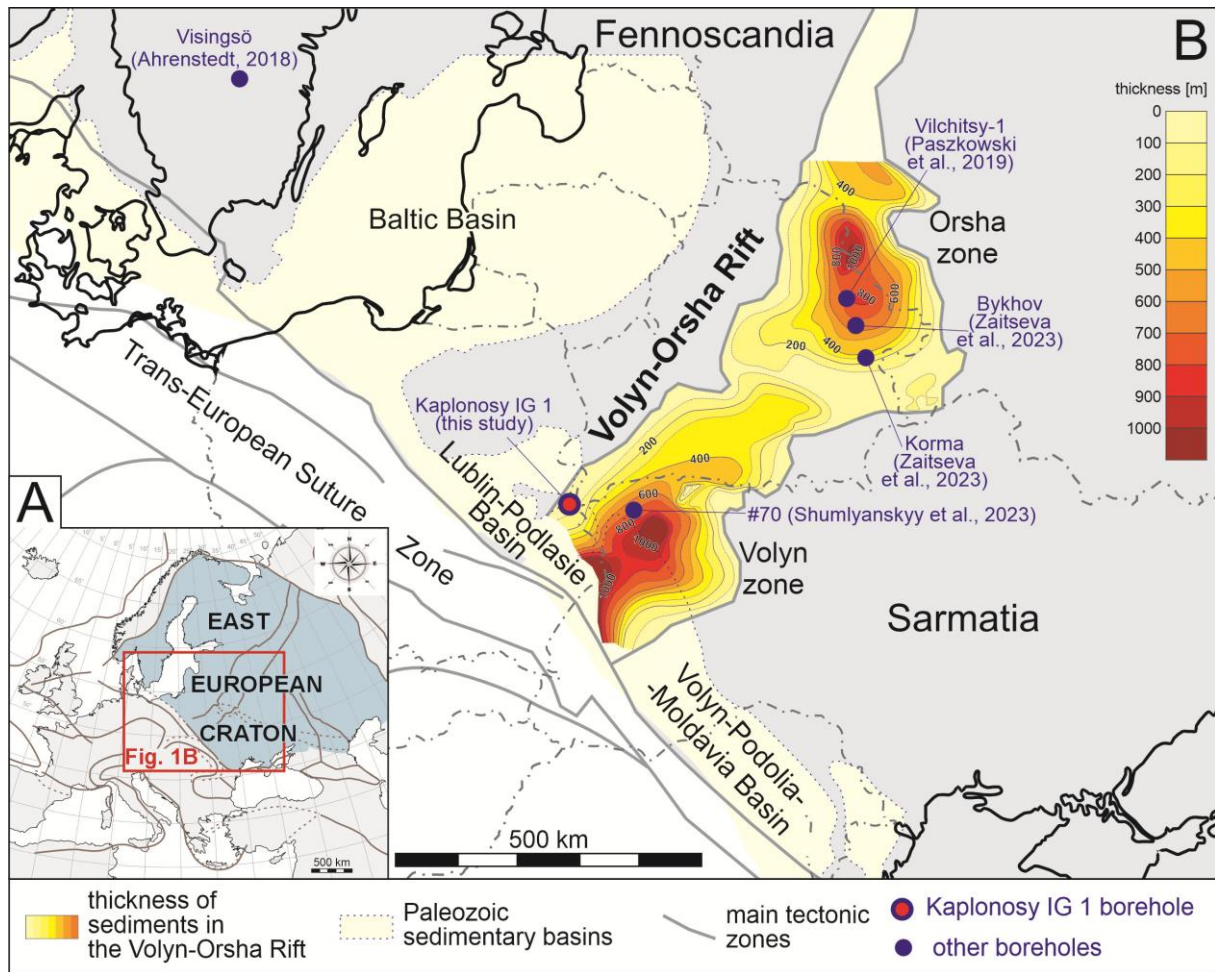
Fig. 1. Location of the Volyn-Orsha Rift and its relation to (A) the East European Craton (EEC) and (B) Lublin-Podlasie Basin (after: Poprawa, 2019, 2020; Krzemińska et al., 2024), together with the location of the studied Kaplonosy IG 1 borehole ( N51^{\circ}37'13,42'' , E23^{\circ}21'24,47'' ). B – the thickness map of the Polesie formation (Poland), in Belarus, including the Pinsk, Orsha, and Lapici formations, is compiled from the data of Gareckij et al. (1987) and Wichrowska (1992). The location of boreholes for which similar U-Pb dating on detrital zircon from the Polissia Group were conducted (Paszowski et al., 2019; Shumlyanskyy et al., 2023; Zaitseva et al., 2023) and Neoproterozoic Visingsö Group of southern Sweden (Moczyłowska et al., 2017; Ahrenstedt) are also indicated.
