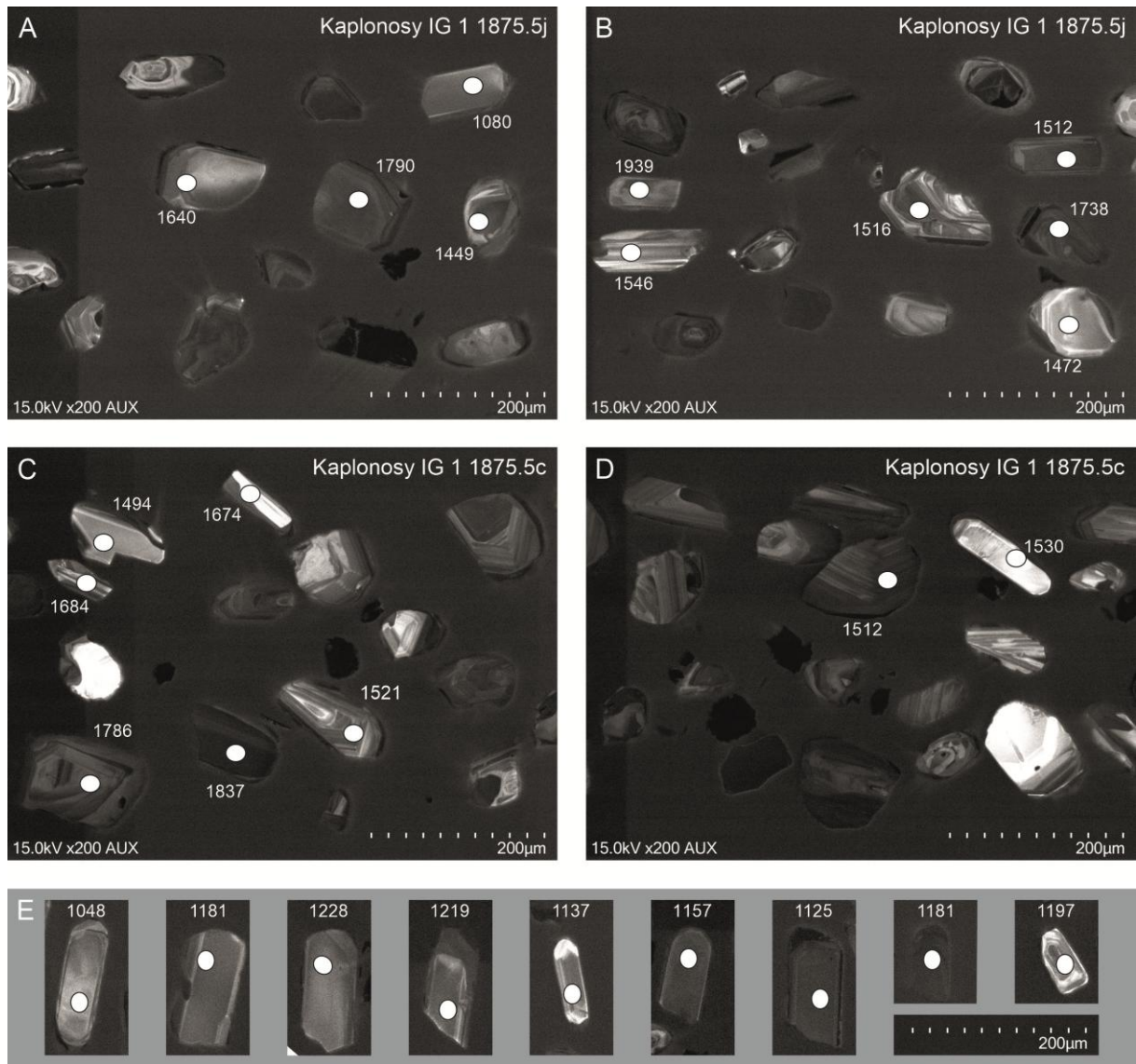
Fig. 5. The characteristics of representative detrital zircon grains disclosed by cathodoluminescence imaging CL, accompanied with selected images of single zircons representing a relatively youngest age group. The morphology of some grains is visible in the transmitted light photos. SHRIMP analyses are located and labelled with their ^{207}\text{Pb}/^{206}\text{Pb} ages.
