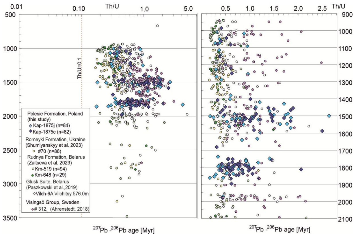
Fig. 9. Comparisons of detrital zircon ages and Th/U parameter based on data from this study and data taken from Ahrenstend (2018); Paszkowski et al. (2019); Zaitseva et al. (2023); Shumlyanskyy et al. (2023)
