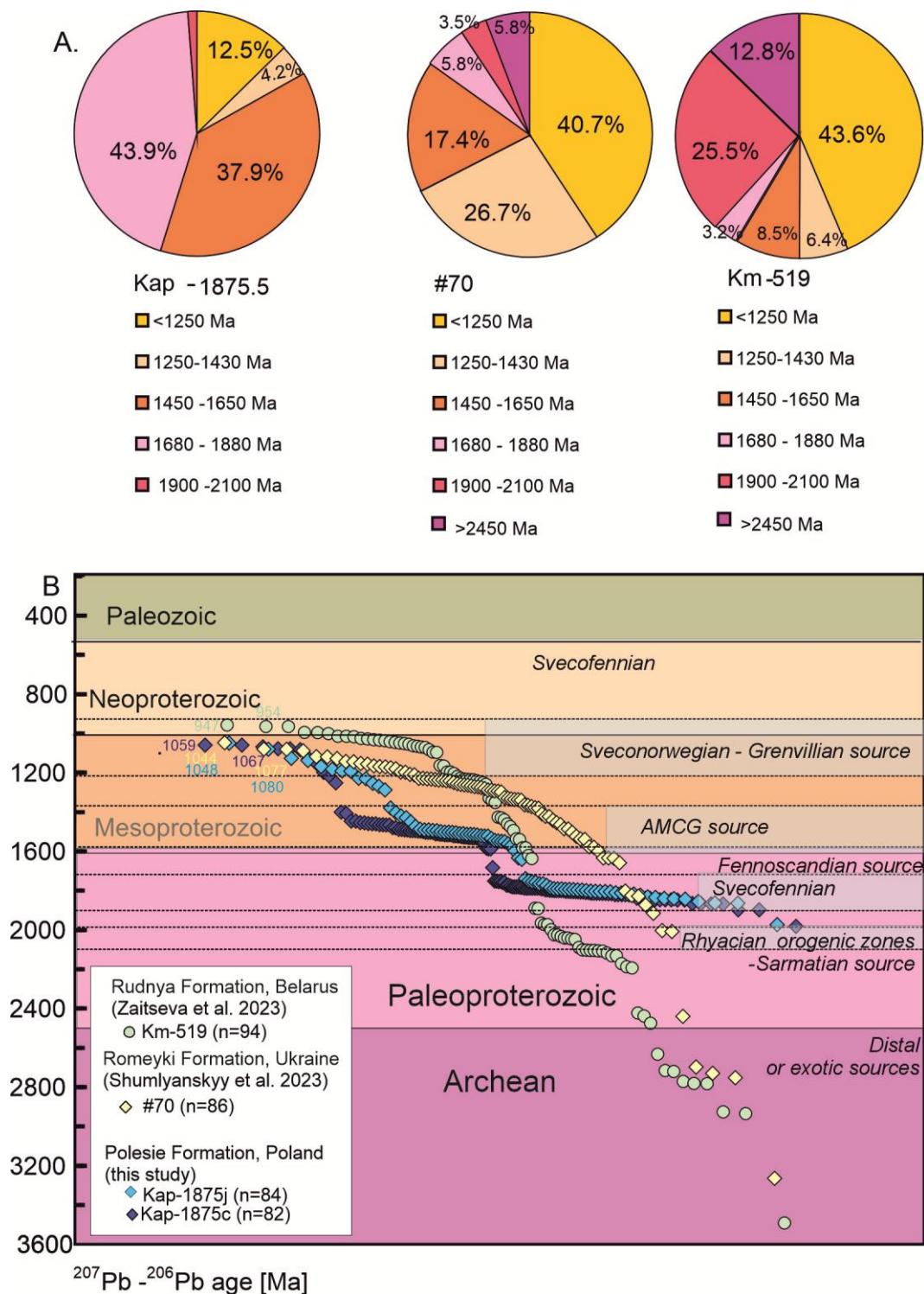
Fig. 13. Schematic diagram including a comparison of detrital zircon ages of the early Neoproterozoic cratonic sandstones from lower part of VOR: (A). pie chart graphics showing the proportion of the zircon Pb-Pb ages according to the time frames matched to the source areas and rocks; B. Linearized-probability plot diagram showing a distribution of detrital components within distinct parts of VOR; Generalized potential source areas and rocks are indicated. Data after Zaitseva et al. (2023) - sample Km-519; after Shumlyanskyy et al. (2023) - sample #70; Sample Kap-1875.5 merged (this study).
