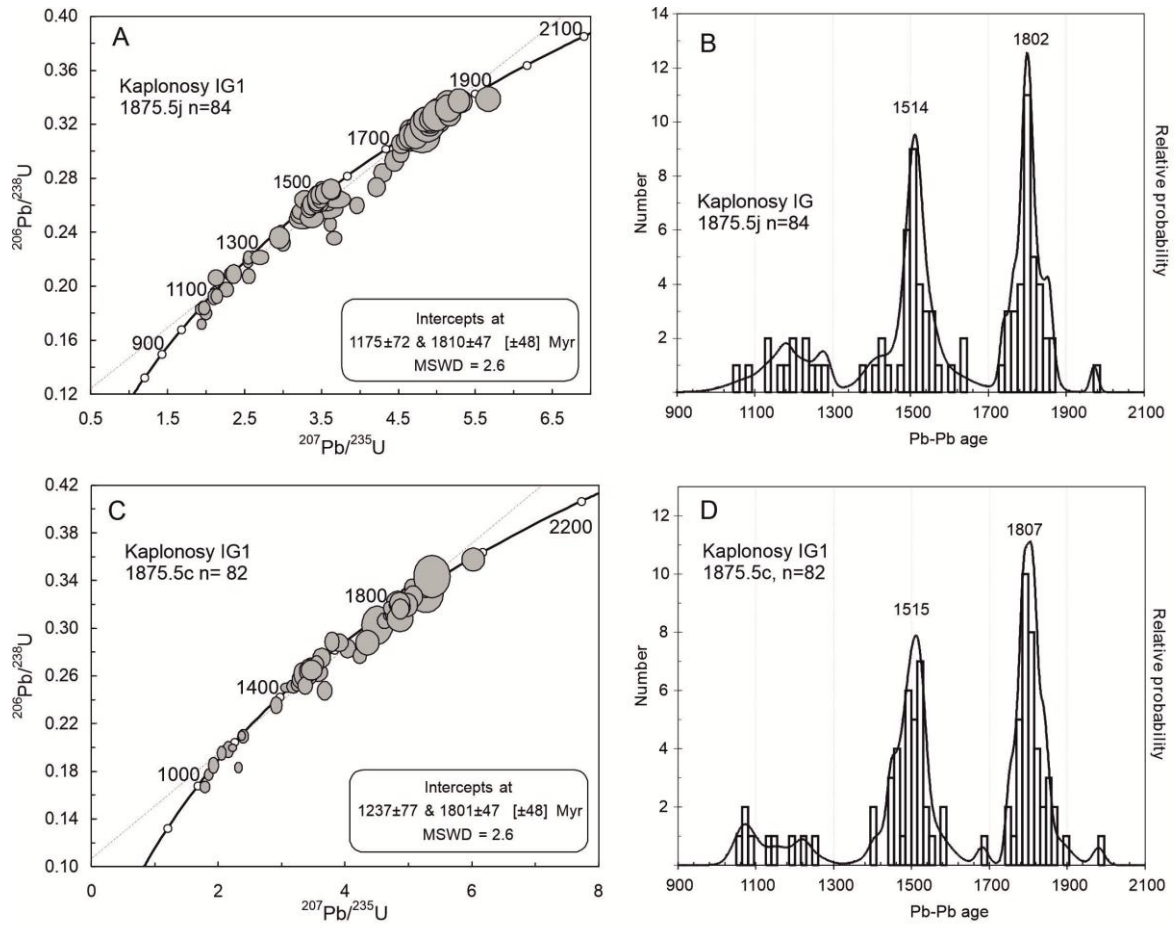
Fig. 6. Results of the SHRIMP U-Pb dating of detrital zircons of the Polesie formation Kap-1875.5 Concordia diagrams and Probability density plot (PDP) diagrams, displaying ages from the main zircon populations in the analyzed sub-samples.
