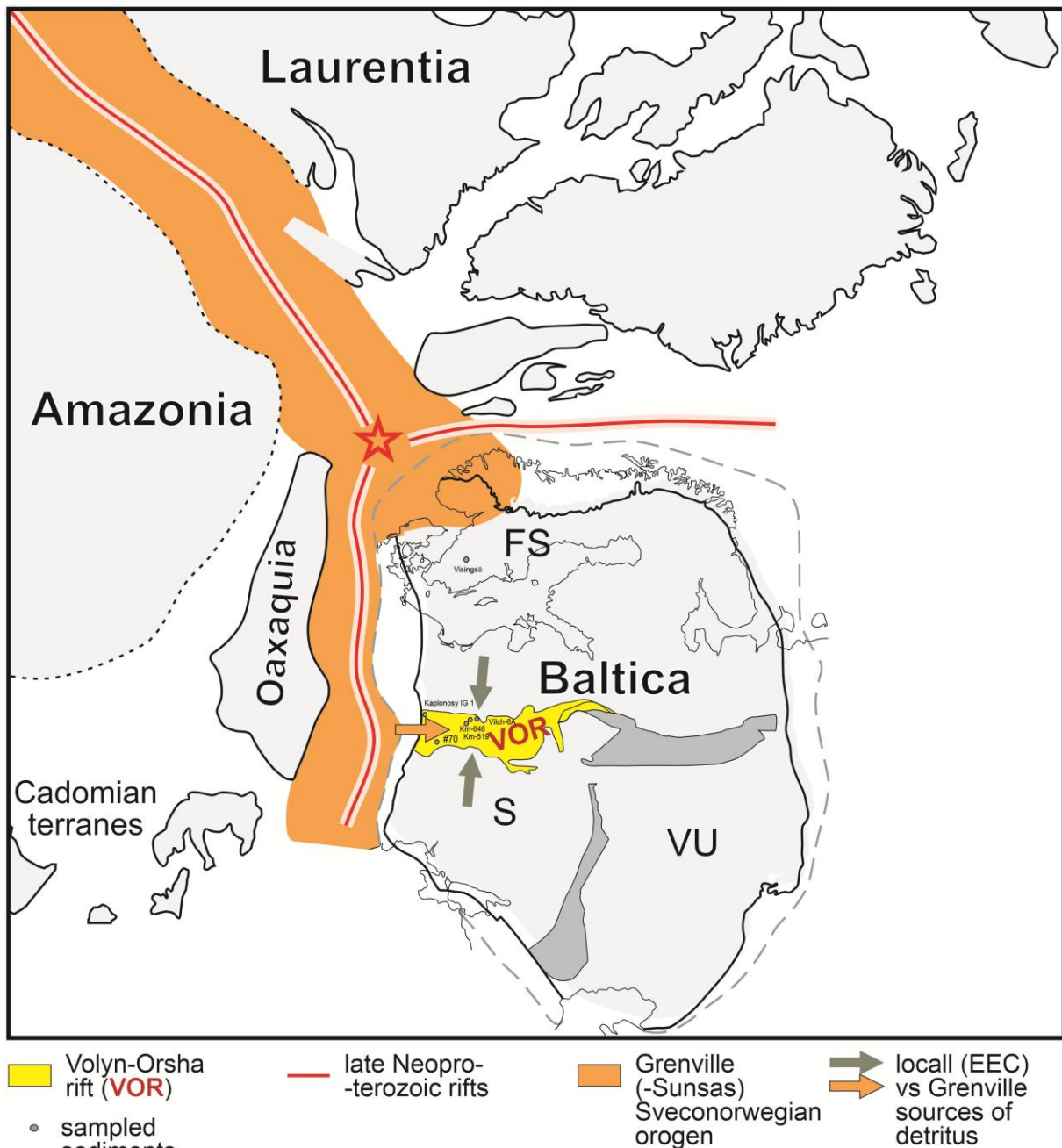
Fig. 11. Supposed palaeogeographic position of source areas of detritus for the Polesie formation relative to the position of the Orsha-Volyn Rift. The basin was supplied with detritus from both the Grenville-Sunas-Sveconorwegian orogen to the west of the Baltica, and the local cratonic sources. FS: Fennoscandia, S: Sarmatia, VU: Volgo-Uralia blocks.
