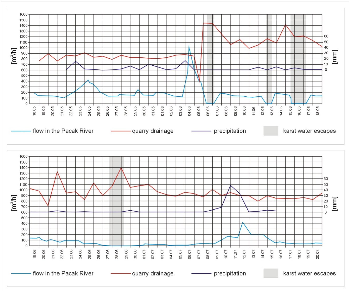
Fig. 13. Episodes revealing response of the gypsum karst aquifer and the Pacak River to increased rainfall recharge (1976)
