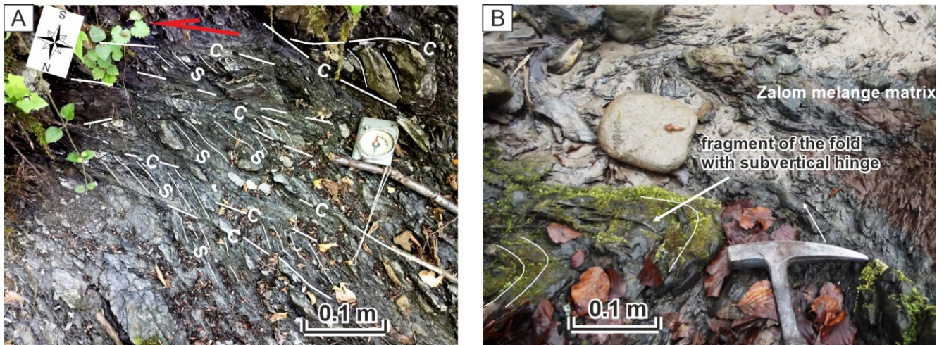
Fig. 25. Zalom mélangé near the contact zone between Burkut and Dukla units (Zalom Stream between the villages of Polyana and Uklin)
