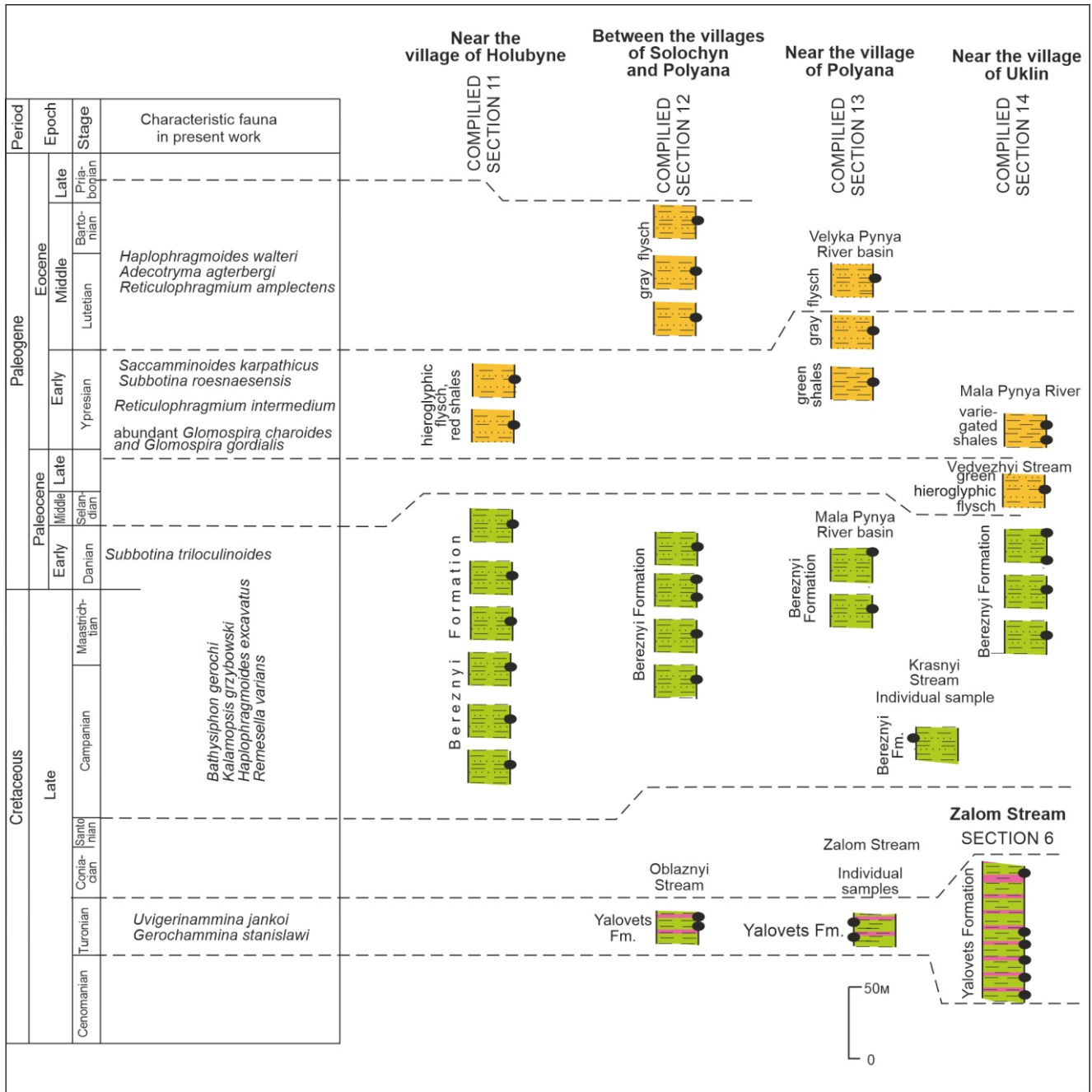
Fig. 18. The age, correlation and characteristic foraminifera of the Yalovets Formation (Turonian), Bereznyi Formation (Senonian-Paleocene) and hieroglyphic-type deposits (Paleocene-Eocene), Dukla Unit, Latorytsa River Basin, time scale after Gradstein et al. (2020)
