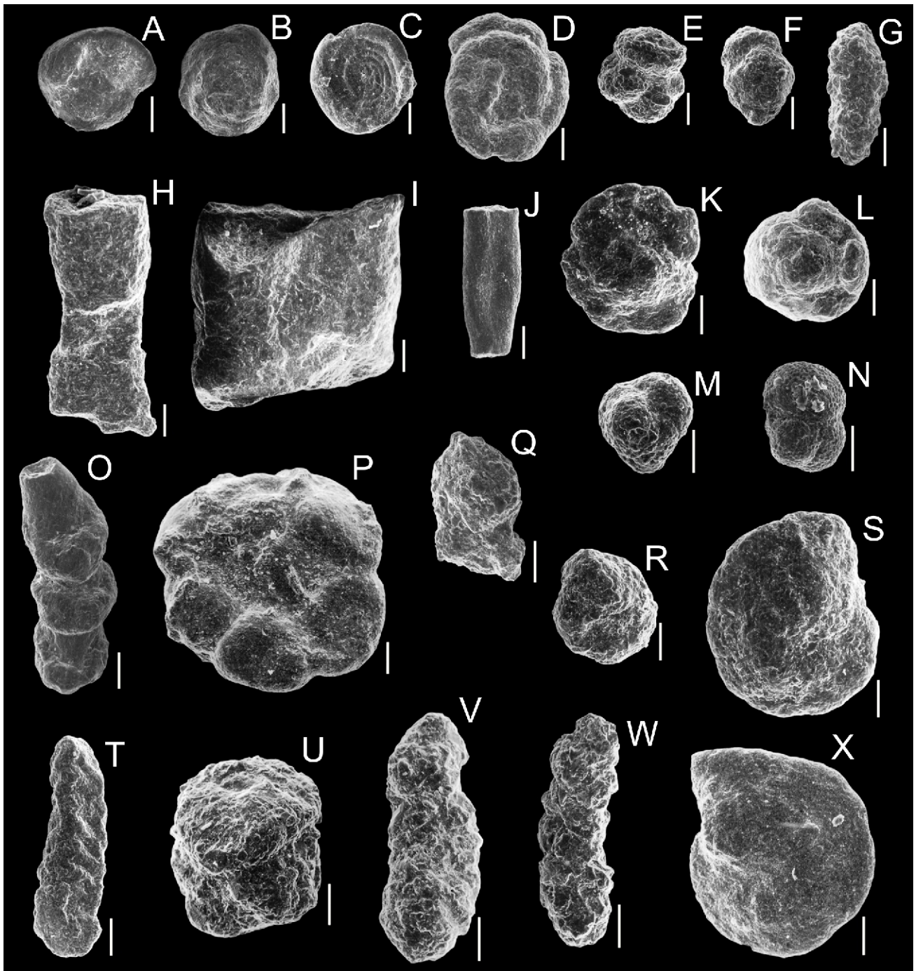
Fig. 19. Foraminifera from deposits of the Dukla Unit
