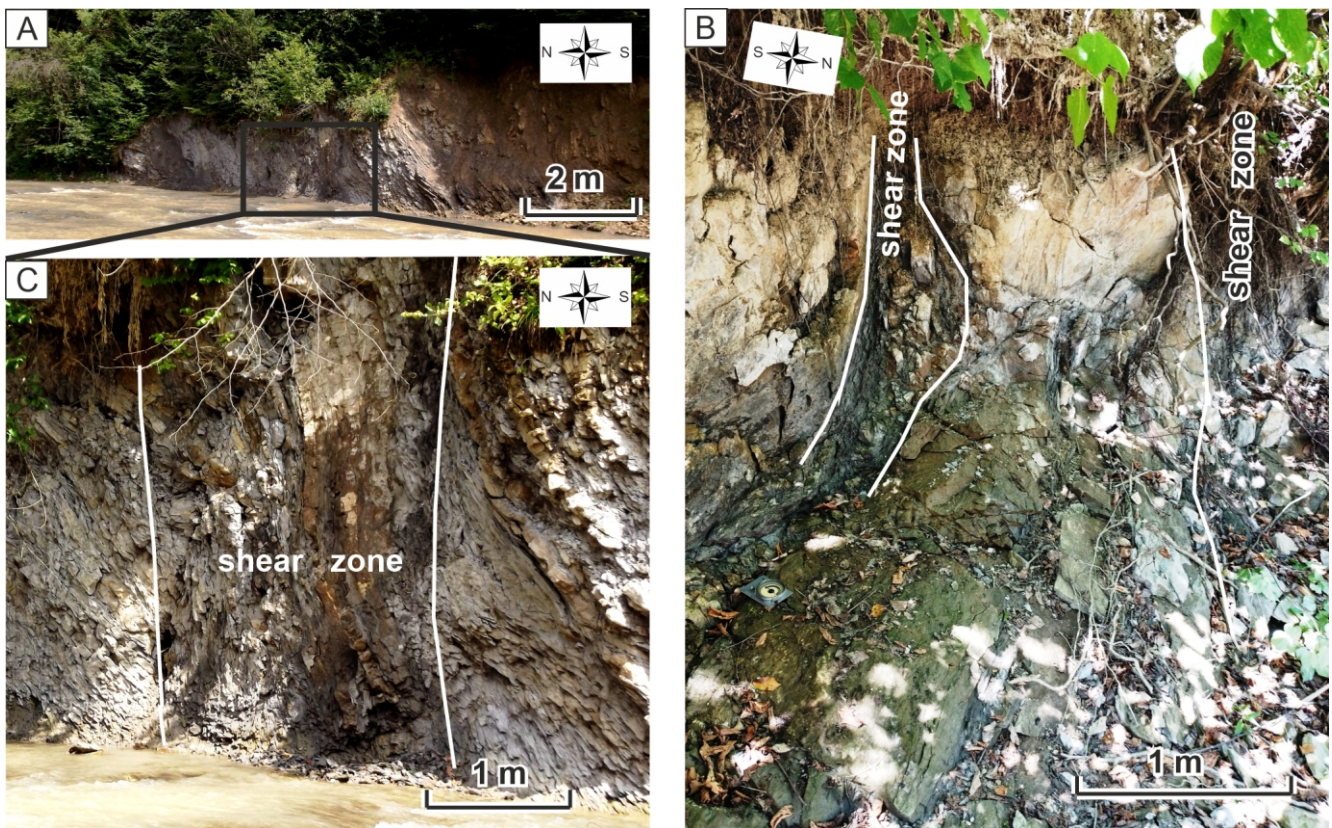
Fig. 26. Shear zones near the contact of the Burkut and Dukla units
