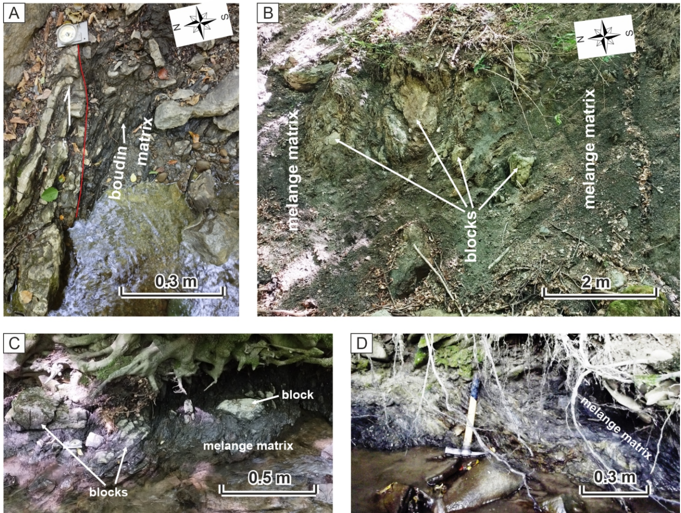
Fig. 23. Broken formations and mélanges near the contact zone of the Eastern Carpathian Svydovets Unit with both the Silesian Unit (A–C) and the Western Carpathian Dukla Unit (D)
