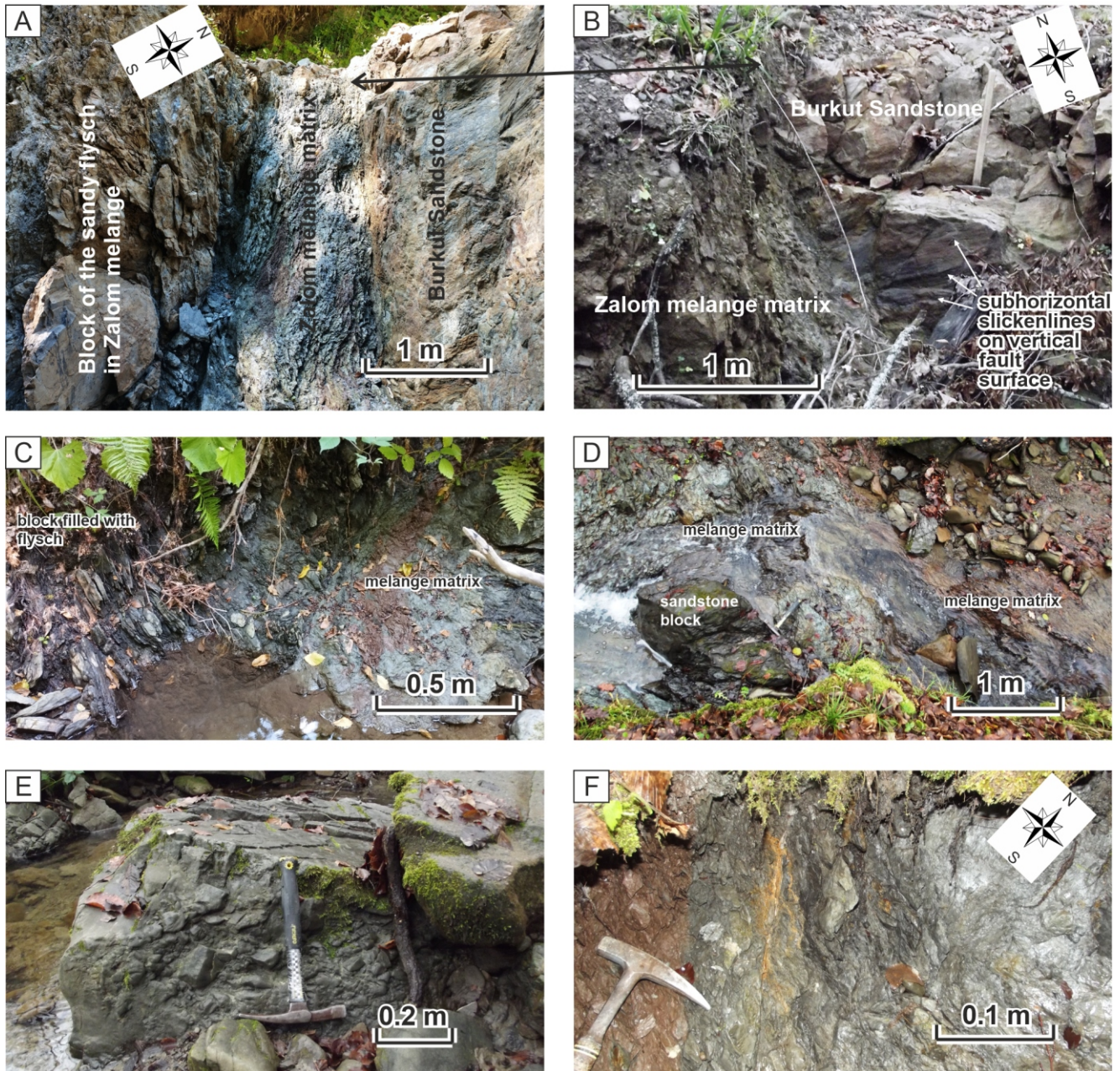
Fig. 24. Zalom mélange near the contact zone between the Eastern Carpathian Burkut Unit and the Western Carpathian Dukla Unit (Zalom Stream between the villages of Polyana and Uklin)
