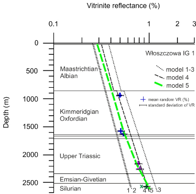
Fig. 5. The mean vitritine reflectance data vs. calculated models for the Włoszczowa IG 1 borehole section
