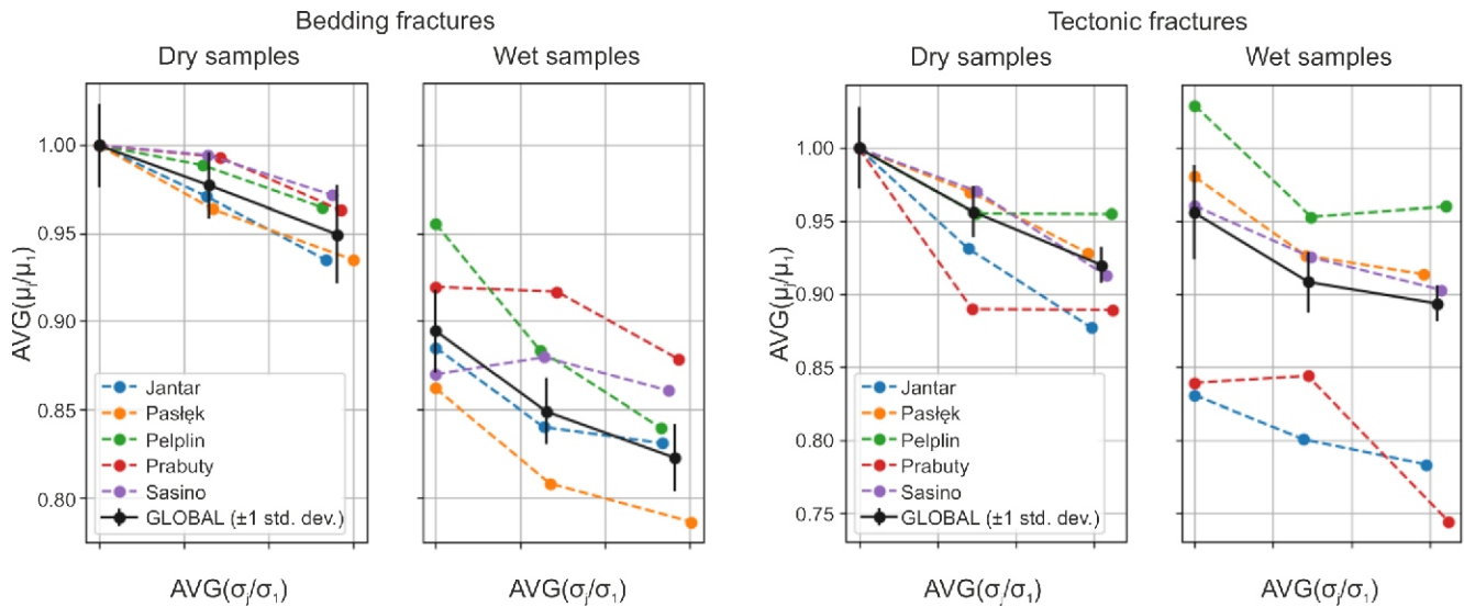
Fig. 10. Cross-plots of the friction coefficient and normal load changes in successive load steps, both calibrated to the mean values for the first load step
