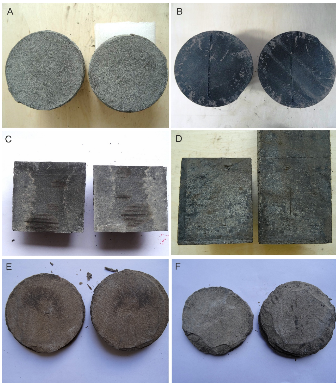
Fig. 2. Examples of the fracture surfaces analysed: A, B – bedding fractures; C, D – tectonic fractures; E, F – tuffite/bentonite bedding planes
