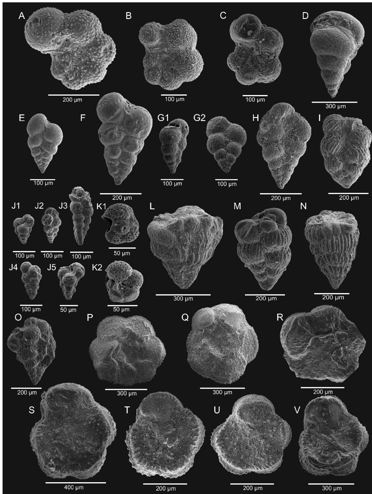
Fig. 3. SEM images of selected planktonic foraminifera from the Hyzne section
