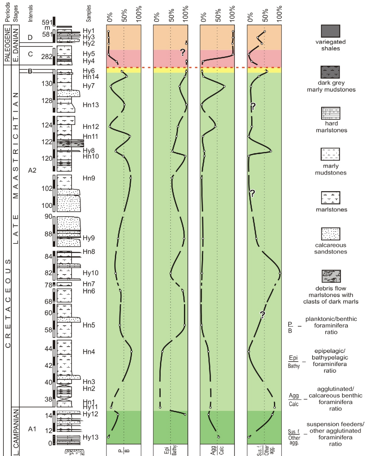
Fig. 8. Quantitative analysis of foraminiferal assemblages of the studied samples
