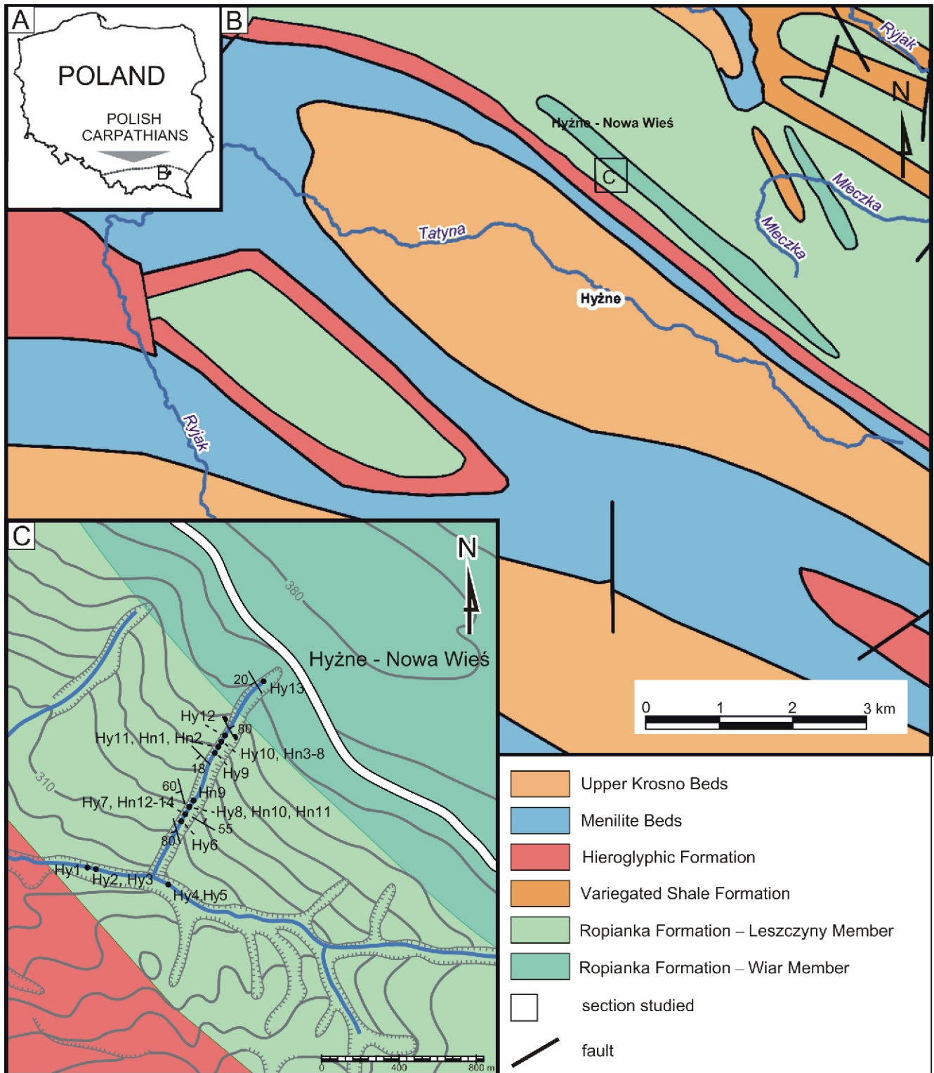
Fig. 1. Location maps of Hyżne section
