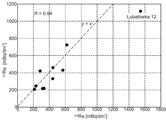
Fig. 5. 226 Ra concentration vs. 224 Ra concentration in the water samples
