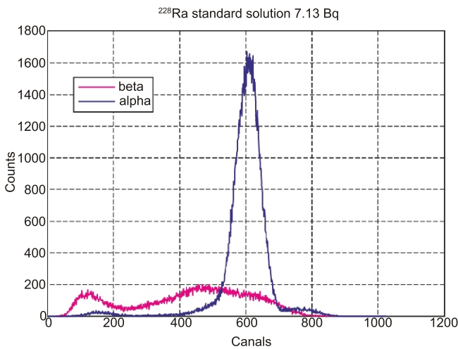
Fig. 2. Alpha and beta spectra of the ^{228}\text{Ra} standard solution measured by Wallac Winspectral 1414 alpha and beta liquid scintillation counter at 50 h elapsed from the radium precipitation
