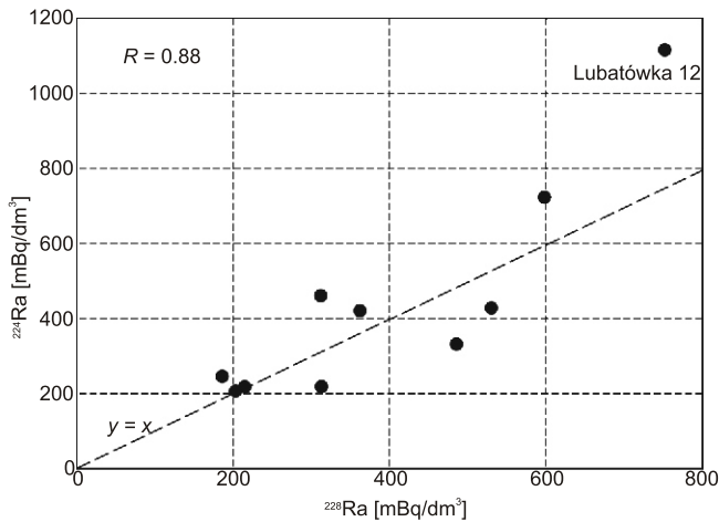
Fig. 6. 228 Ra concentration vs. 224 Ra concentration in water samples
