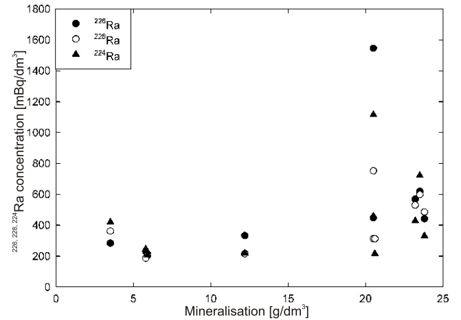
Fig. 8. Activity concentrations of radium isotopes ( 224 Ra, 226 Ra and 228 Ra) vs. TDS in the water samples
