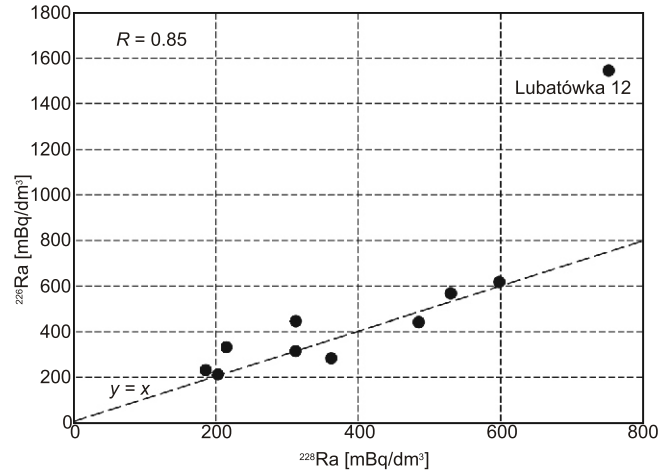
Fig. 7. 226 Ra concentration vs. 228 Ra concentration in the water samples
