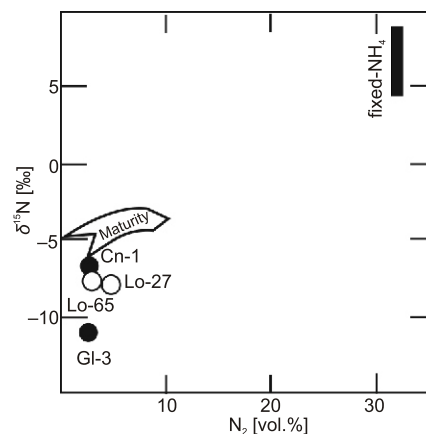
Fig. 17. ^{15}\text{N}(\text{N}_2) versus \text{N}_2 concentration of natural gas accumulated in the Middle and Upper Devonian reservoirs of the study area
