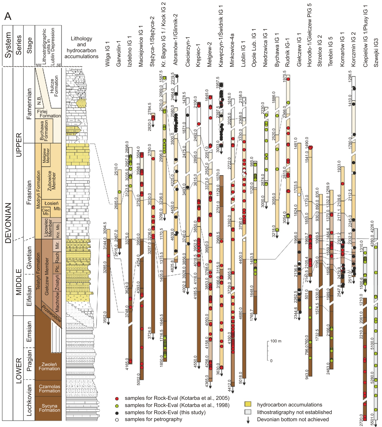
Fig. 3A – stratigraphy, correlation and hydrocarbon potential of the Devonian in the Lublin Basin with location of the samples hydrocarbon accumulations after Helcel-Weil and Dzięgiełowski (2003); B – stratigraphy, correlation and hydrocarbon potential stratigraphy and lithology after Pomyanovskaya (1974);
