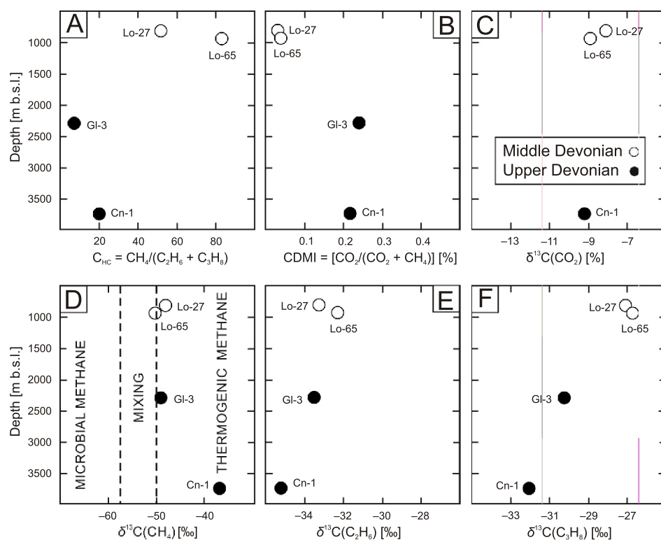
Fig. 15A – hydrocarbon index; B – carbon dioxide-methane index; C – ^{13}\text{C}(\text{CO}_2) ; D – ^{13}\text{C}(\text{CH}_4) ; E – ^{13}\text{C}(\text{C}_2\text{H}_6) ; F – ^{13}\text{C}(\text{C}_3\text{H}_8) versus depth of natural gas accumulated in the Middle and Upper Devonian reservoirs of the study area
