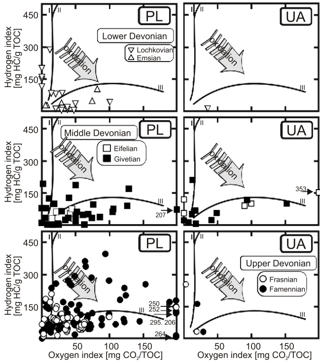
Fig. 7. Rock-Eval hydrogen index versus oxygen index (maturity paths of individual kerogen types after Espitalié et al., 1985)
