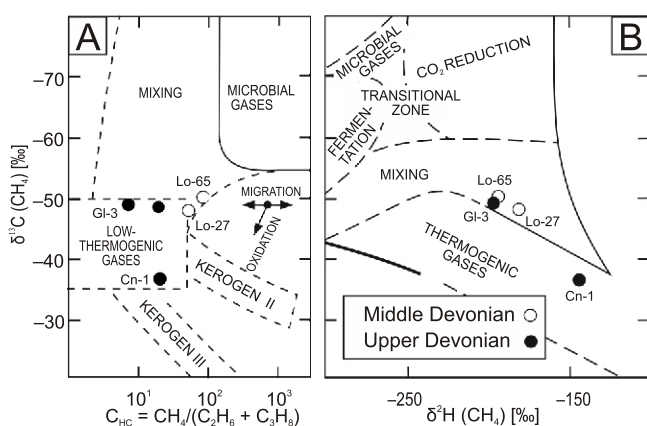
Fig. 12. 13 C of methane versus (A) hydrocarbon index C HC (i.e., CH 4 /(C 2 H 6 + C 3 H 8 )) and (B) 2 H(CH 4 ) for the natural gas accumulated in the Middle and Upper Devonian reservoirs of the study area
