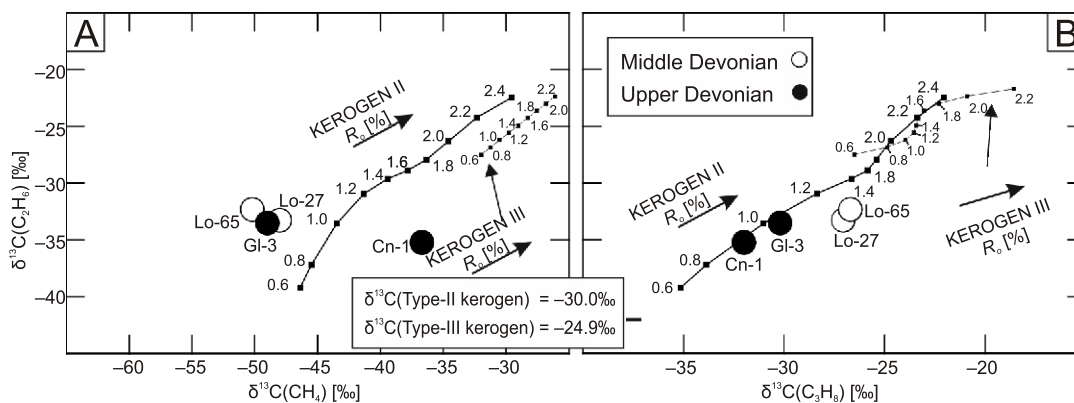
Fig. 13. ^{13}\text{C}(\text{C}_2\text{H}_6) versus (A) ^{13}\text{C}(\text{CH}_4) and (B) ^{13}\text{C}(\text{C}_3\text{H}_8) for natural gas accumulated in the Middle and Upper Devonian reservoirs of the study area
