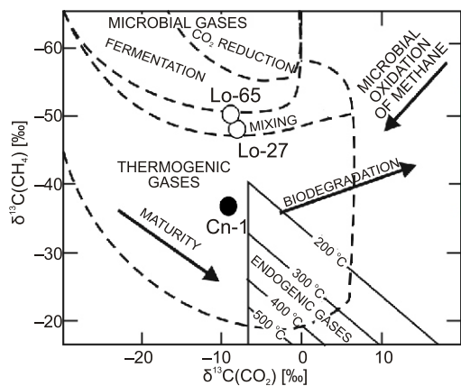
Fig. 16. ^{13}\text{C}(\text{CH}_4) versus ^{13}\text{C}(\text{CO}_2) for natural gas accumulated in the Middle and Upper Devonian reservoirs of the study area
